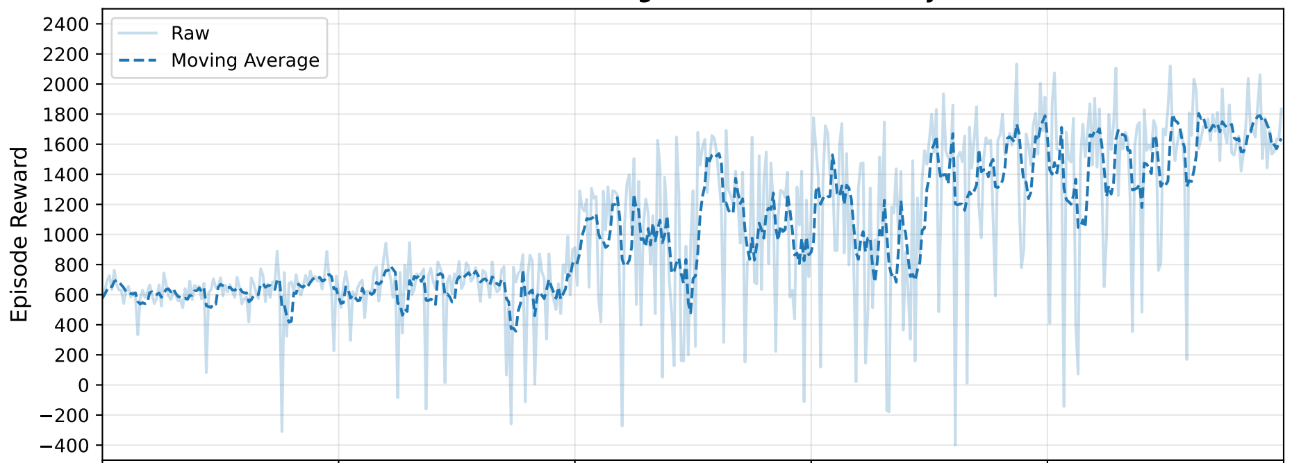
Reward Convergence - Stall Duration
