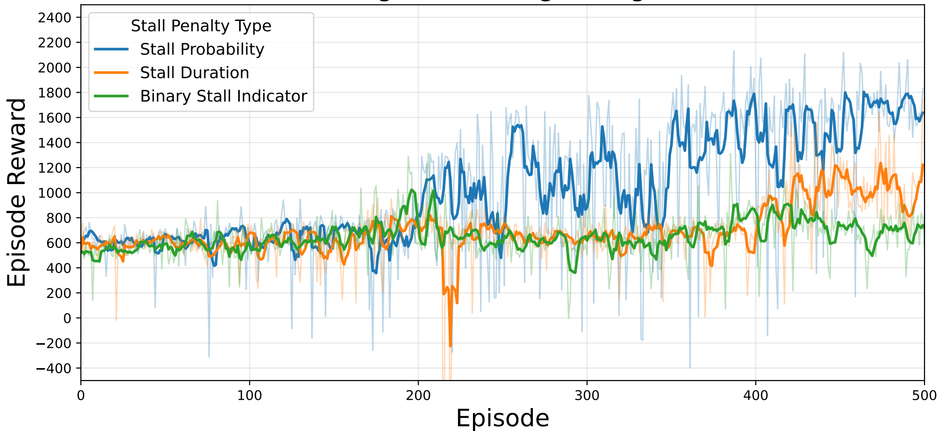
Reward Convergence (Moving Average, window=5)
