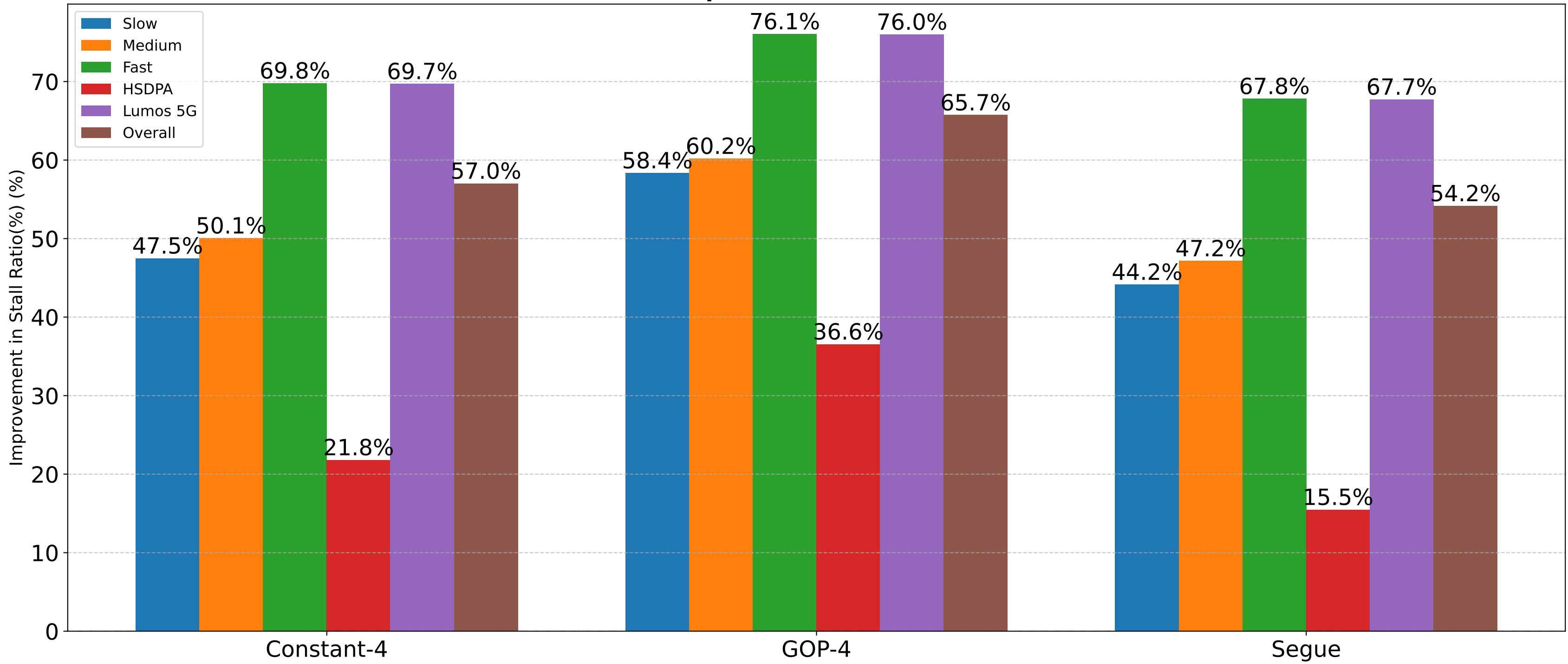
QAOCs Improvement in Stall Ratio(%)
