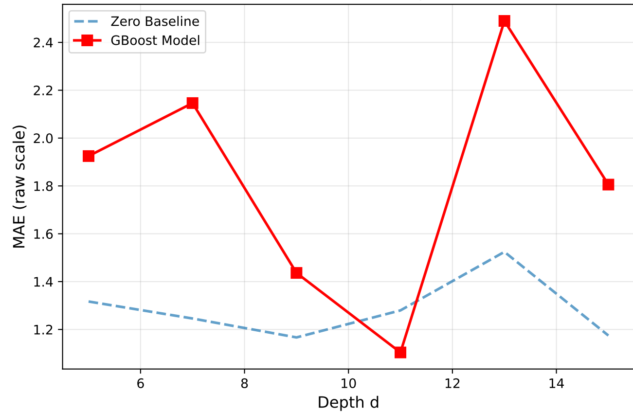
Y2 Prediction: MAE Comparison
