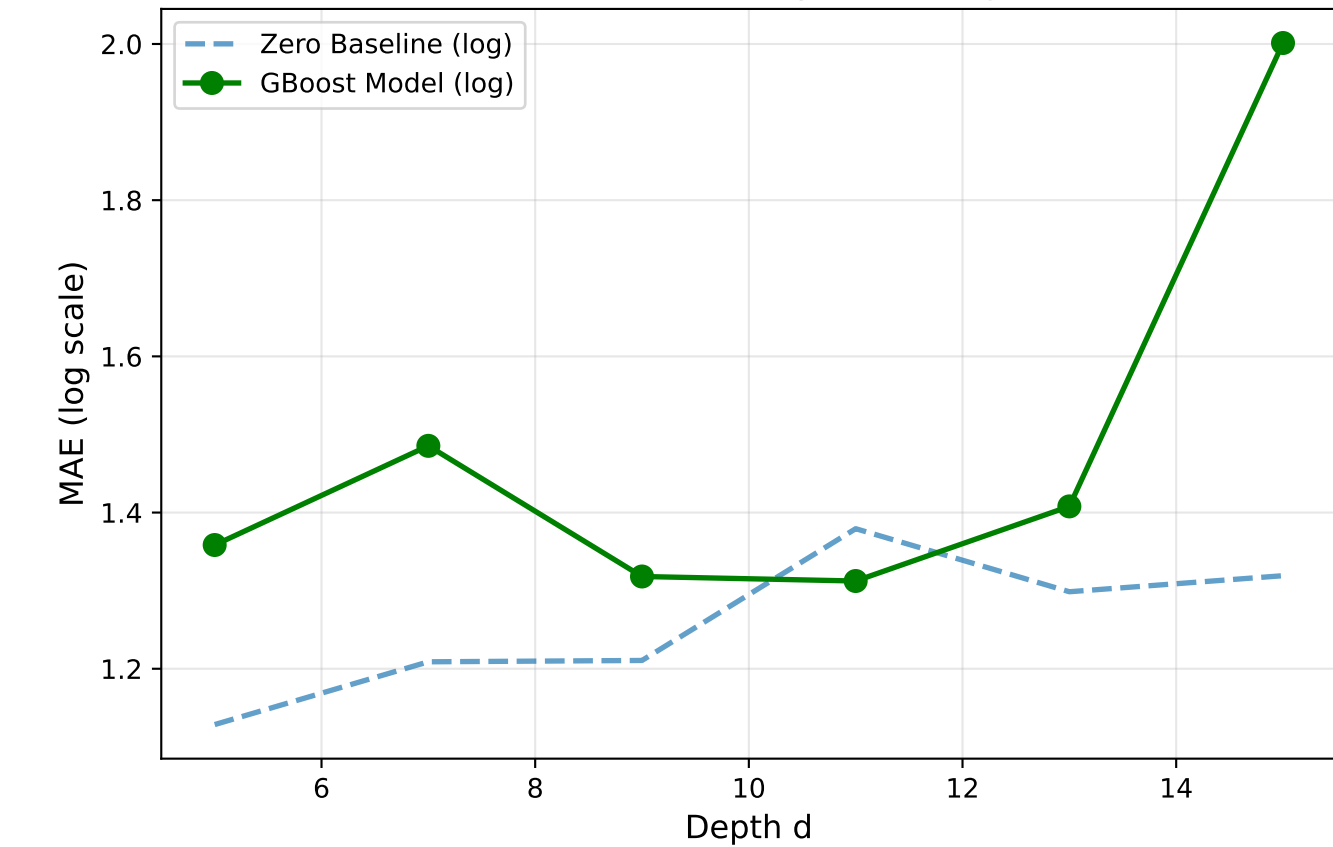
Y1 Prediction: MAE Comparison (log scale)
