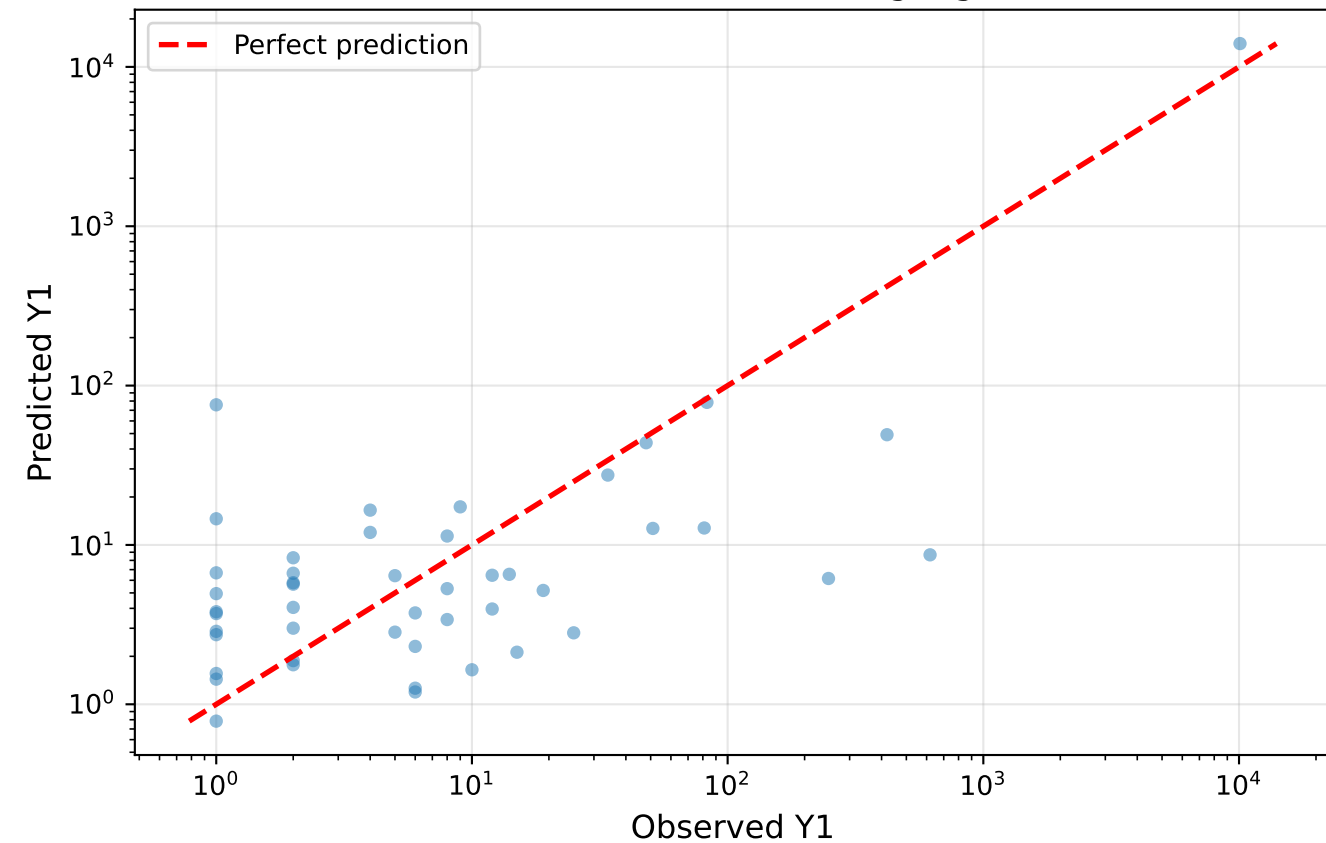
Y1: Observed vs Predicted (log-log scale)
