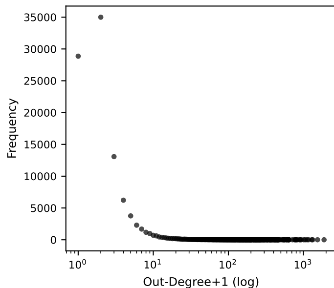
Out-Degree Distribution
