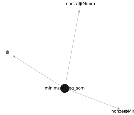
in_degree (low)
