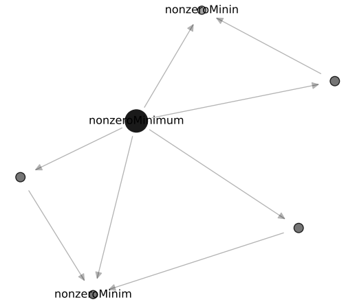
in_degree (low)
