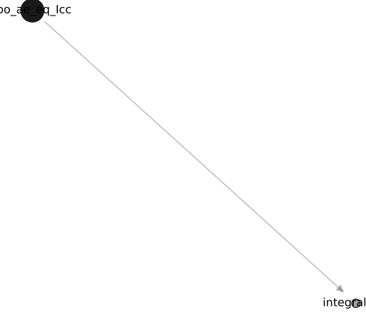
component (high)
