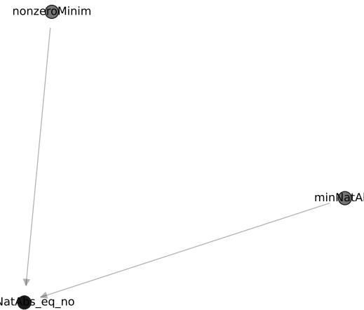
out_degree (low)
