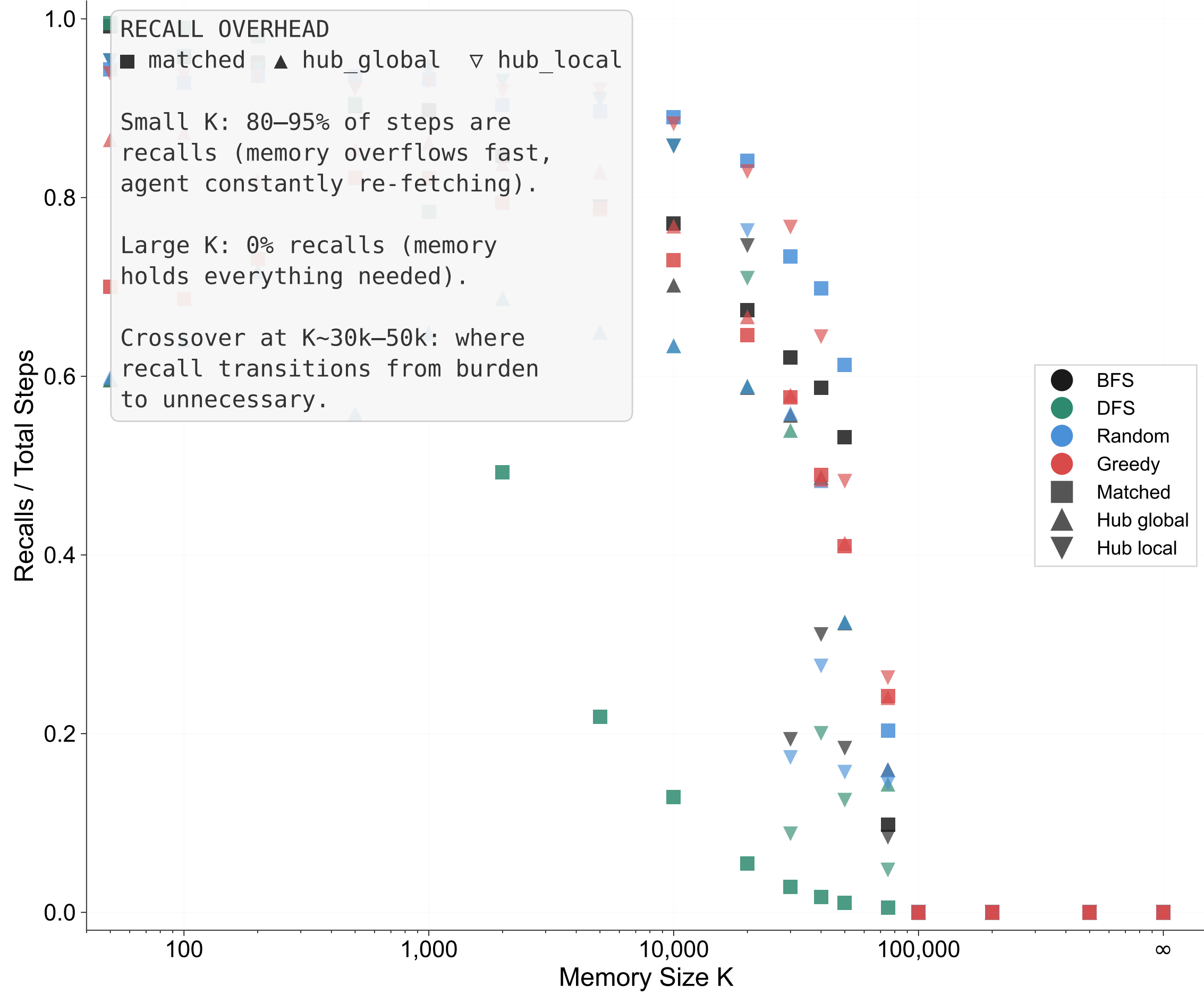
K. Recall Fraction (@60k budget)
