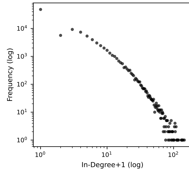
In-Degree Distribution
