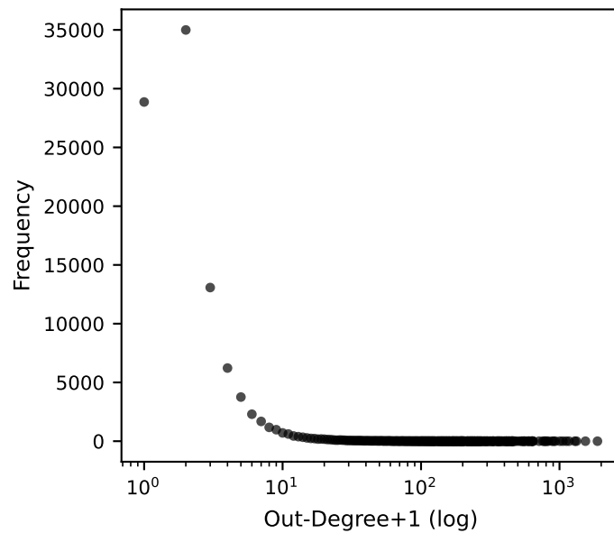
Out-Degree Distribution
