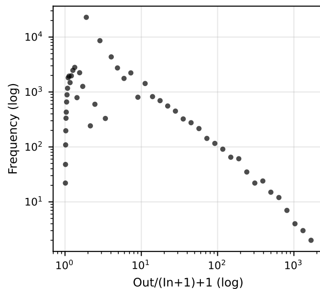
Out/(In+1) Distribution
