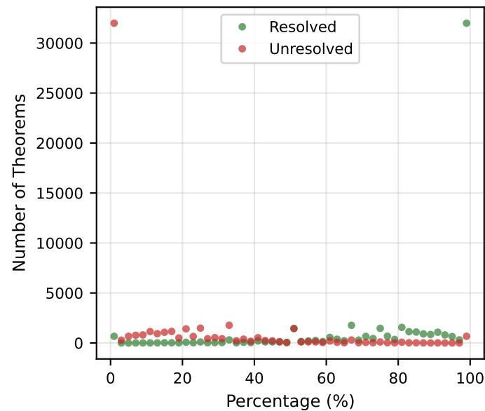
Premise Resolution Rates
