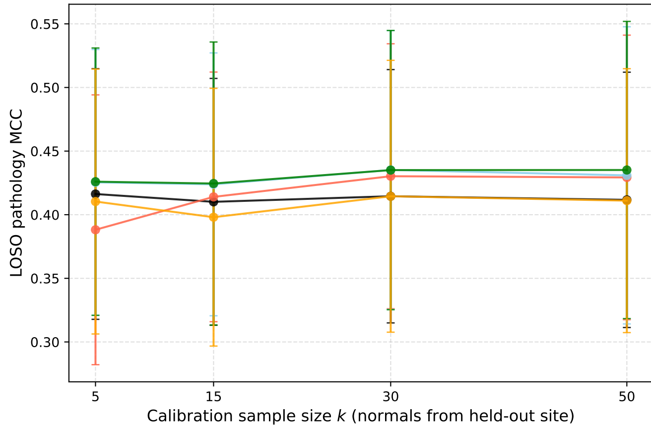
Pathology MCC vs calibration sample size
