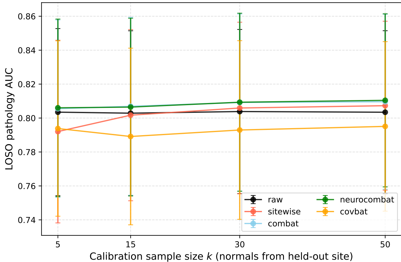
Pathology AUC vs calibration sample size
