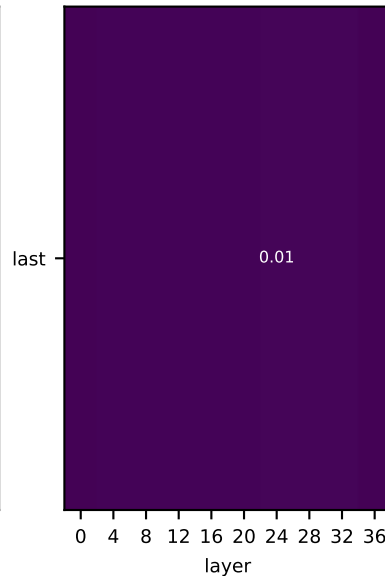
cross-lexeme: control
