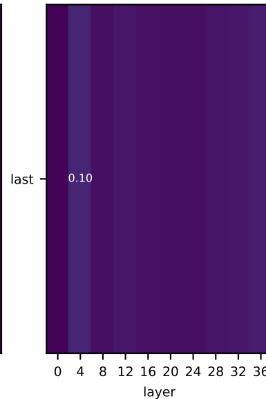
cross-lexeme: selectivity
