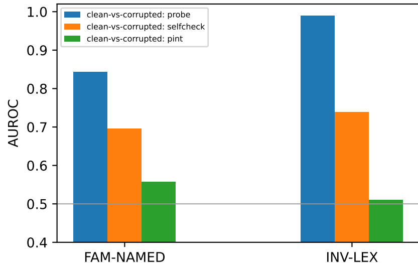
E3.2 dimension-inconsistency detector
