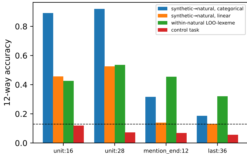
E3.1 naturalistic mentions (Qwen3-4B)
