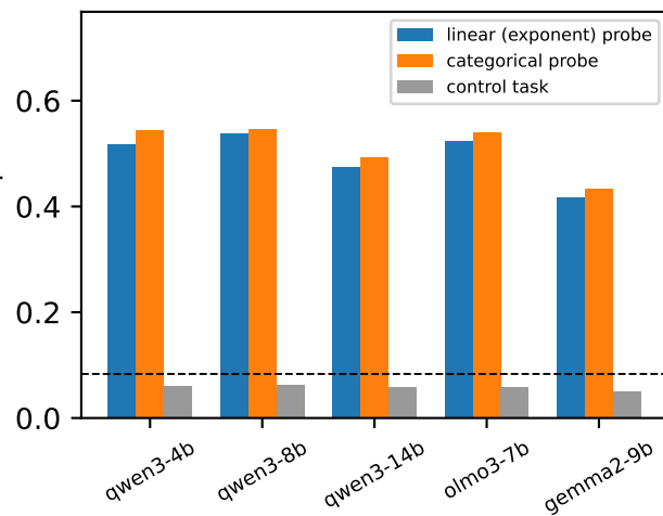
position unit (layer 28)
