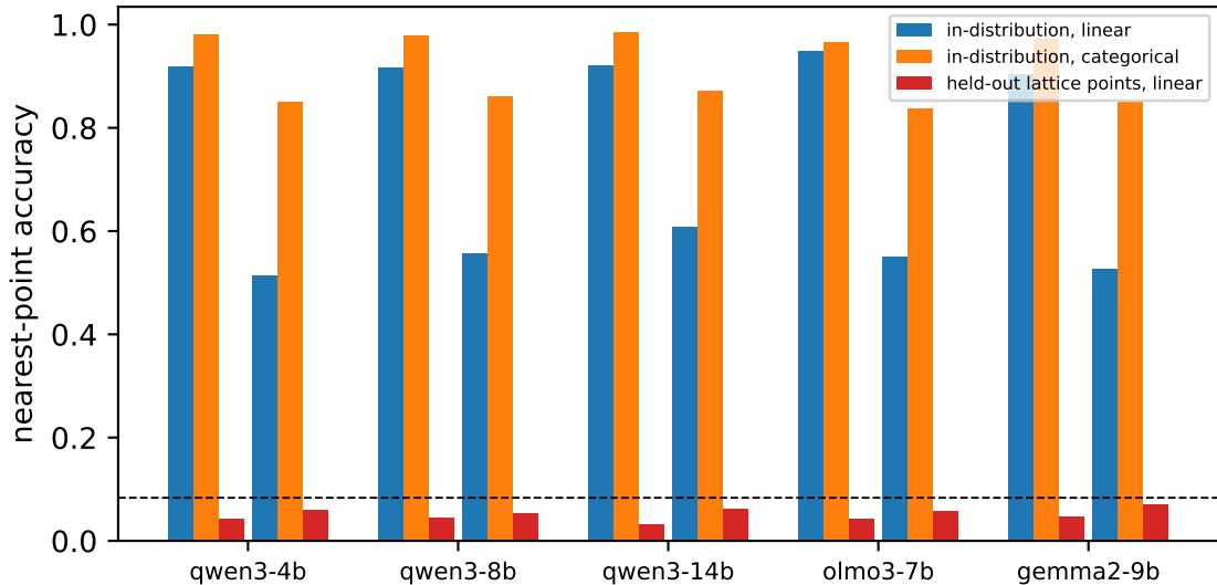
H2: no extrapolation to held-out lattice points (left bars: unit token; right bars: anaphor)
