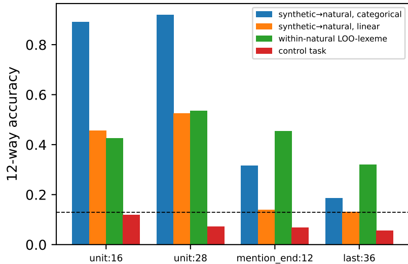
E3.1 naturalistic mentions (Qwen3-4B)
