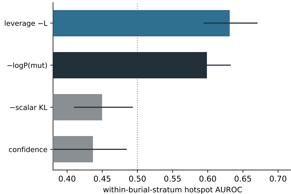
a the mixed derivative adds binding info; confidence barely does b confidence is BELOW chance; leverage predicts
