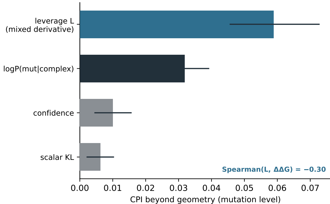
a the mixed derivative adds binding info; confidence barely does b confidence is BELOW chance; leverage predicts
