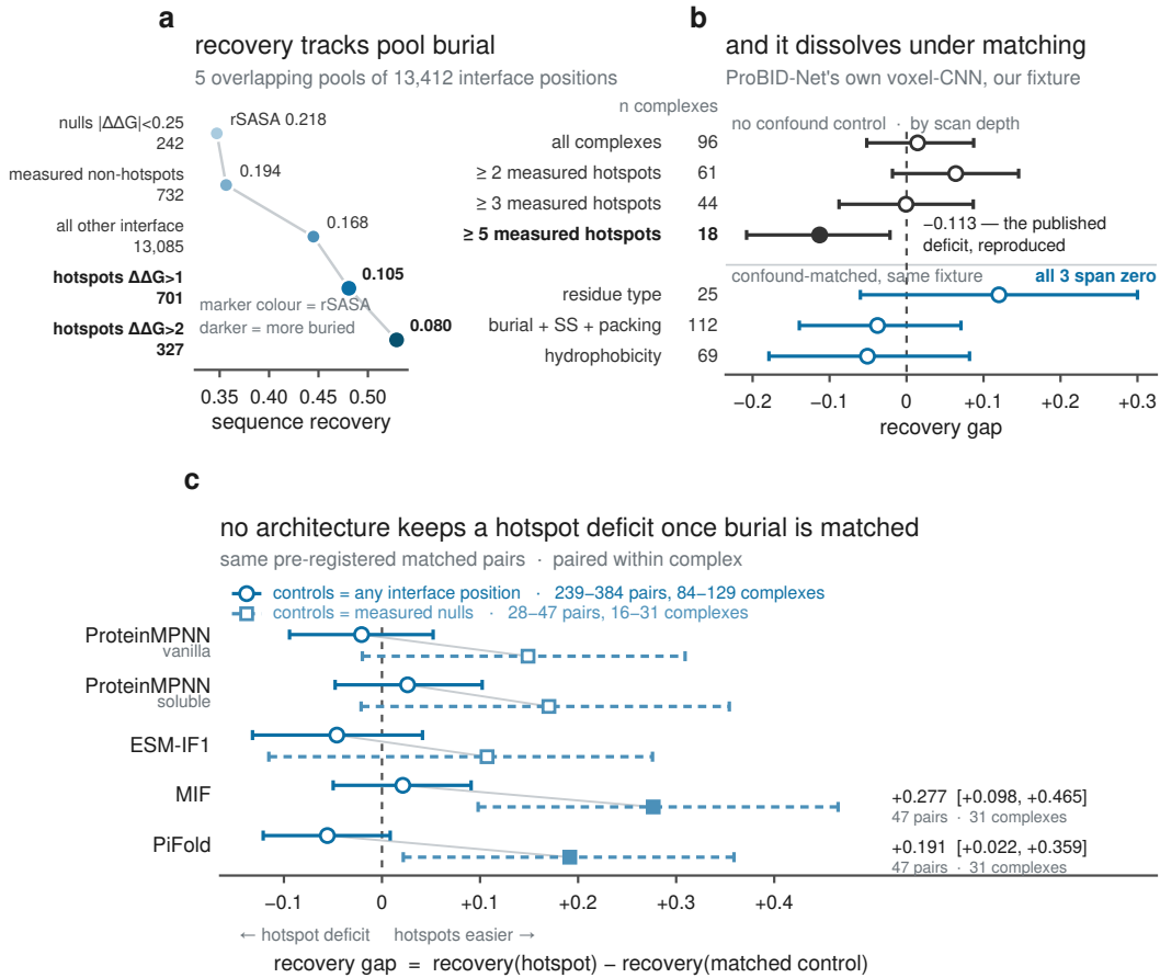
whiskers = 95% complex-clustered bootstrap CI (10,000 replicates, seed 20260803); filled mark = CI excludes zero. \Delta SASA is the one cheap hotspot feature the matching does not control, so it is checked separately: the 384-pair tier carries a \Delta SASA imbalance of +0.072 [+0.045, +0.100], and adjusting the gap for it moves it only -0.042 \rightarrow -0.028 nats.
