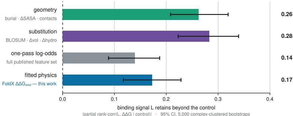
Figure 11: The beyond-X ladder in one matched metric (partial rank-correlation of L with experimental \Delta\Delta G , controlling for each competing feature class). L clears geometry, substitution similarity, the one-pass log-odds, and a fitted physics energy function. Every scalar of P stays at the floor.
