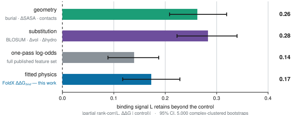
Figure 1: The beyond-X ladder in one matched metric (partial rank-correlation of L with experimental \Delta\Delta G , controlling for each competing feature class). L clears geometry, substitution similarity, the one-pass log-odds, and a fitted physics energy function. Every scalar of P stays at the floor.
