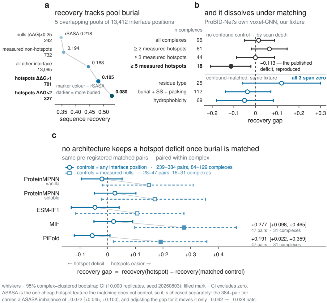
Figure 10: On crystal backbones the hotspot recovery deficit tracks burial. Under the pre-registered matched-pair design it attenuates to statistical indistinguishability, so the published deficit is largely a burial confound.
