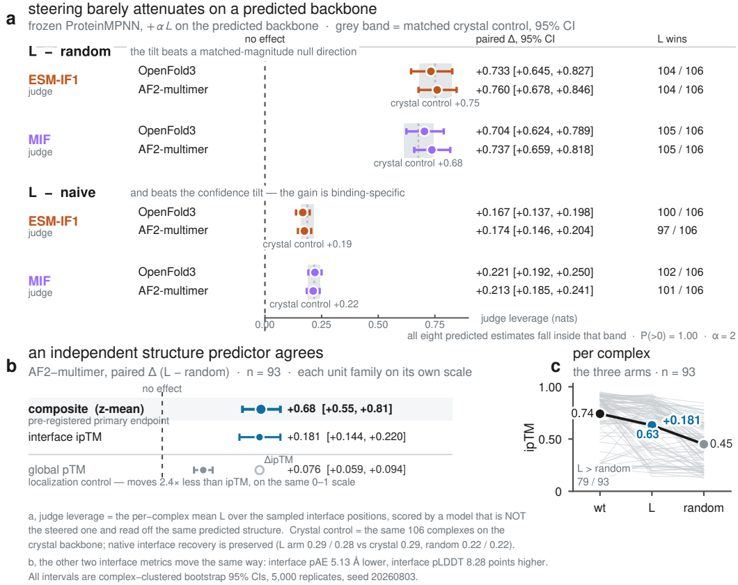
Figure 8: Steering survives the swap to a predicted backbone. a , judge-level paired L – random and L – naive on OpenFold3 and AF2-multimer backbones under two anti-circular judges. The grey band is the matched crystal control’s 95% CI on the same 106 complexes, and all eight predicted estimates fall inside it. b , an instrument outside the inverse-folding family agrees, with global pTM as the localization control. c , the same ipTM effect per complex.
