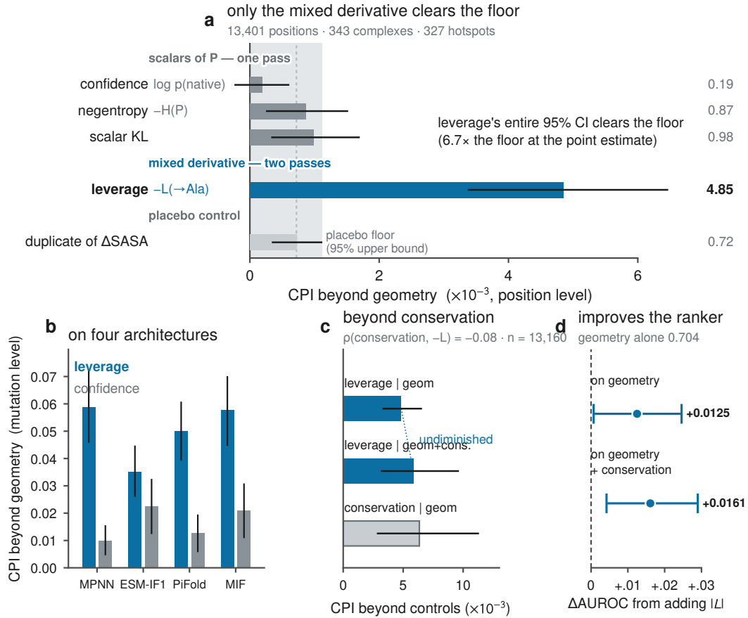
Figure 6: The feature-class law. Every scalar of the bound distribution (confidence, negentropy, the scalar KL) sits at or below the calibrated placebo floor. Only the two-pass mixed derivative clears it.
