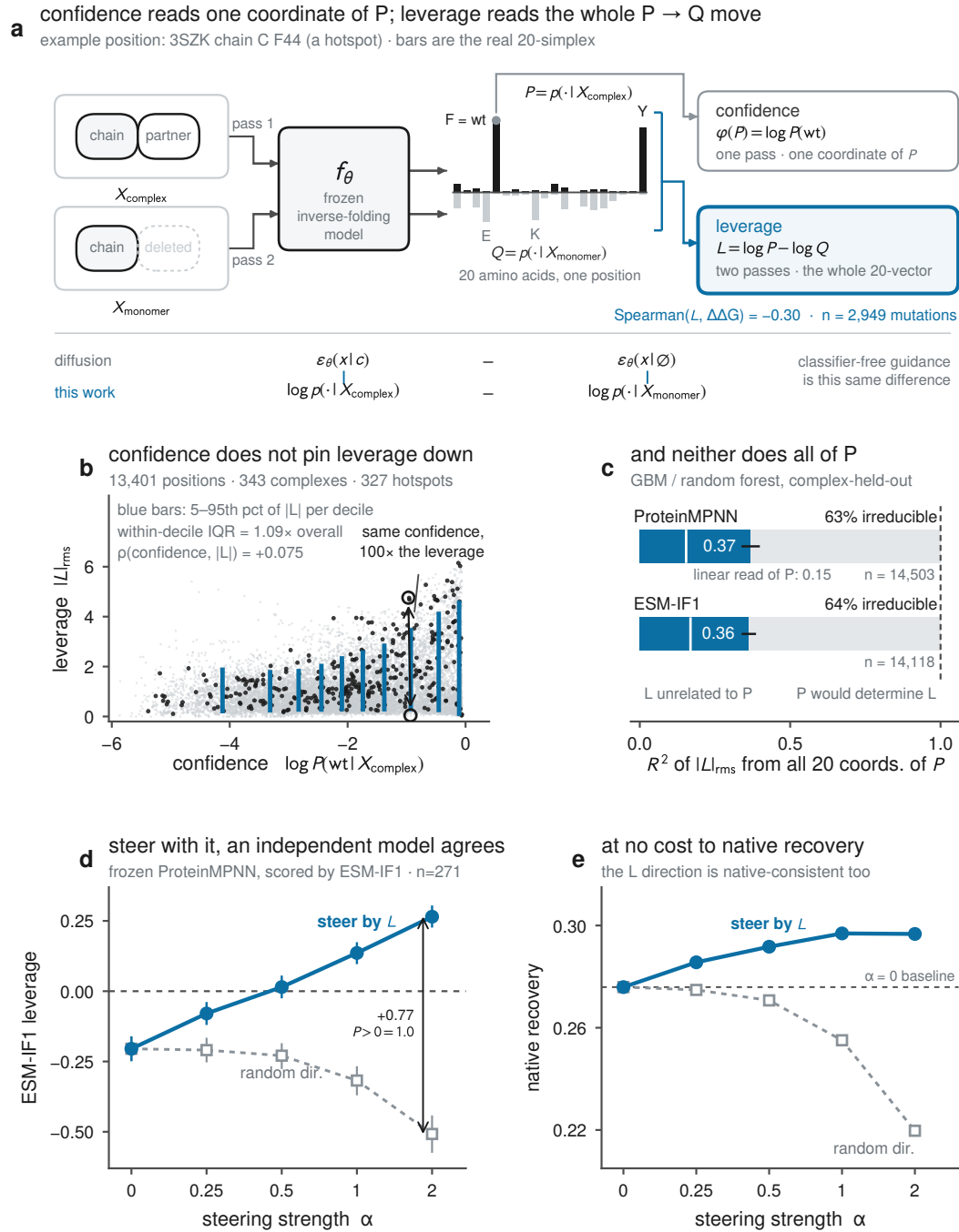
Figure 5: The Confidence-Leverage Decomposition. A flexible learner over the entire bound distribution recovers only about 37 percent of the leverage, so most of the mixed derivative is irreducible from the bound distribution, in both inverse-folding families.
