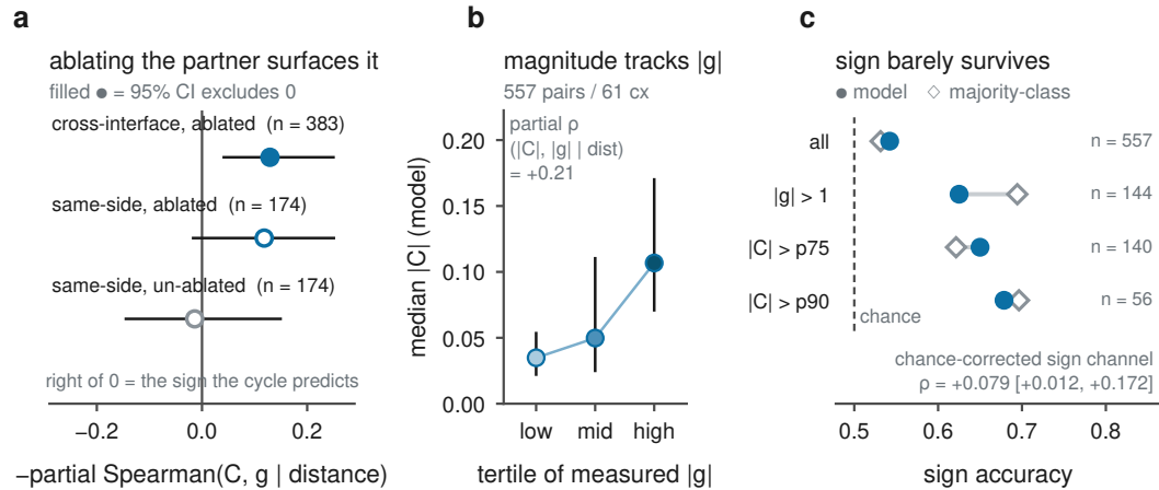
Figure 8: The second mixed derivative. The partner-ablated pairwise coupling tracks measured binding epistasis with the cycle-predicted sign, surviving control for inter-residue distance.
