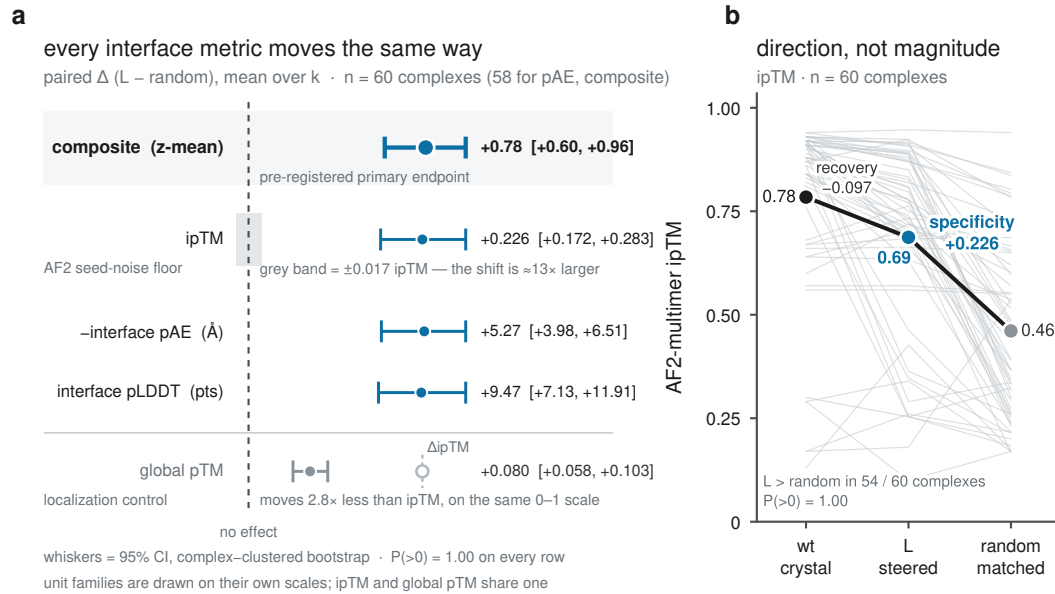
Figure 9: Steering a frozen ProteinMPNN by the mixed derivative raises AF2-multimer interface ipTM against a matched-magnitude random control, and the gain is interface-localized (global pTM rises far less).
