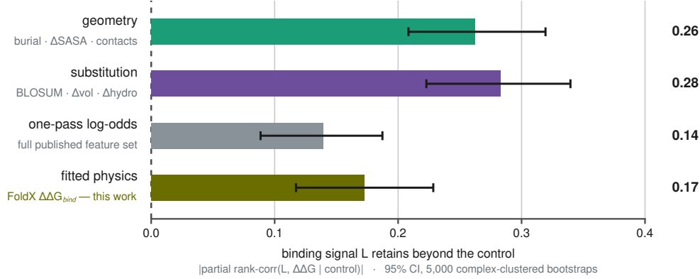
Figure 12: The beyond-X ladder in one matched metric (partial rank-correlation of L with experimental \Delta\Delta G , controlling for each competing feature class). L clears geometry, substitution similarity, the one-pass log-odds, and a fitted physics energy function. Every scalar of P stays at the floor.
