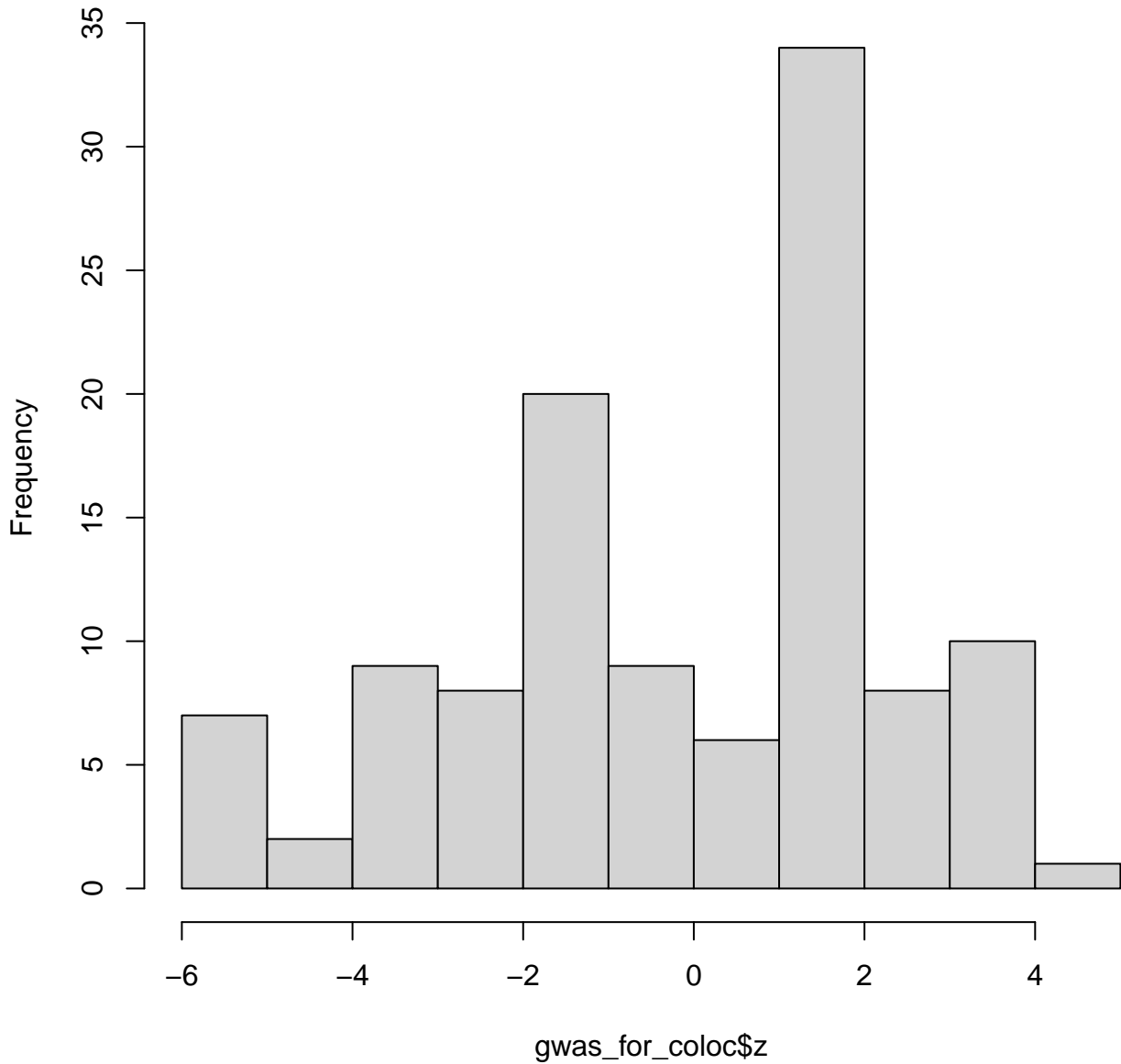
Histogram of gwas_for_coloc$z
