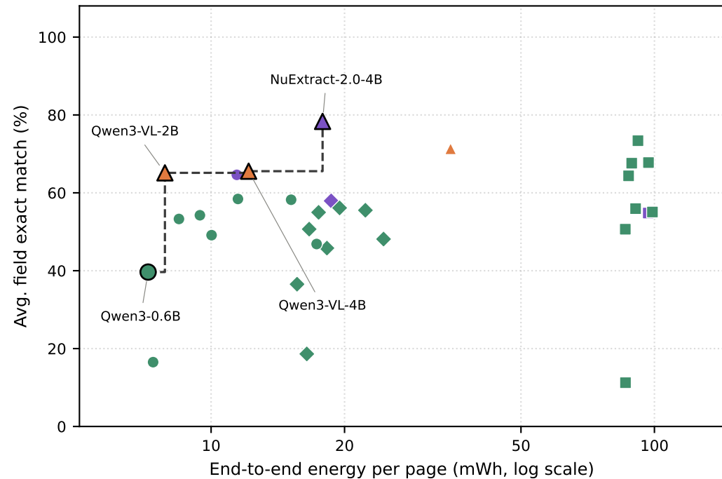
VRDU (scanned, layout-rich)
