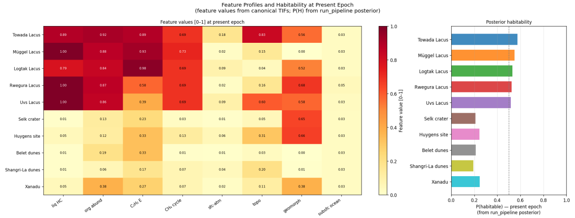
Figure 3.6: Feature profiles and posterior habitability for ten key sites (the leading polar lakes plus equatorial contrast sites, not the full ranking). Left: heatmap of normalised feature values. Right: posterior mean P(H | \mathbf{f}) ; dashed line = prior mean. Selk’s exceptional geodiversity (its standout geomorph column) is clearly visible despite its below-average aggregate score.
