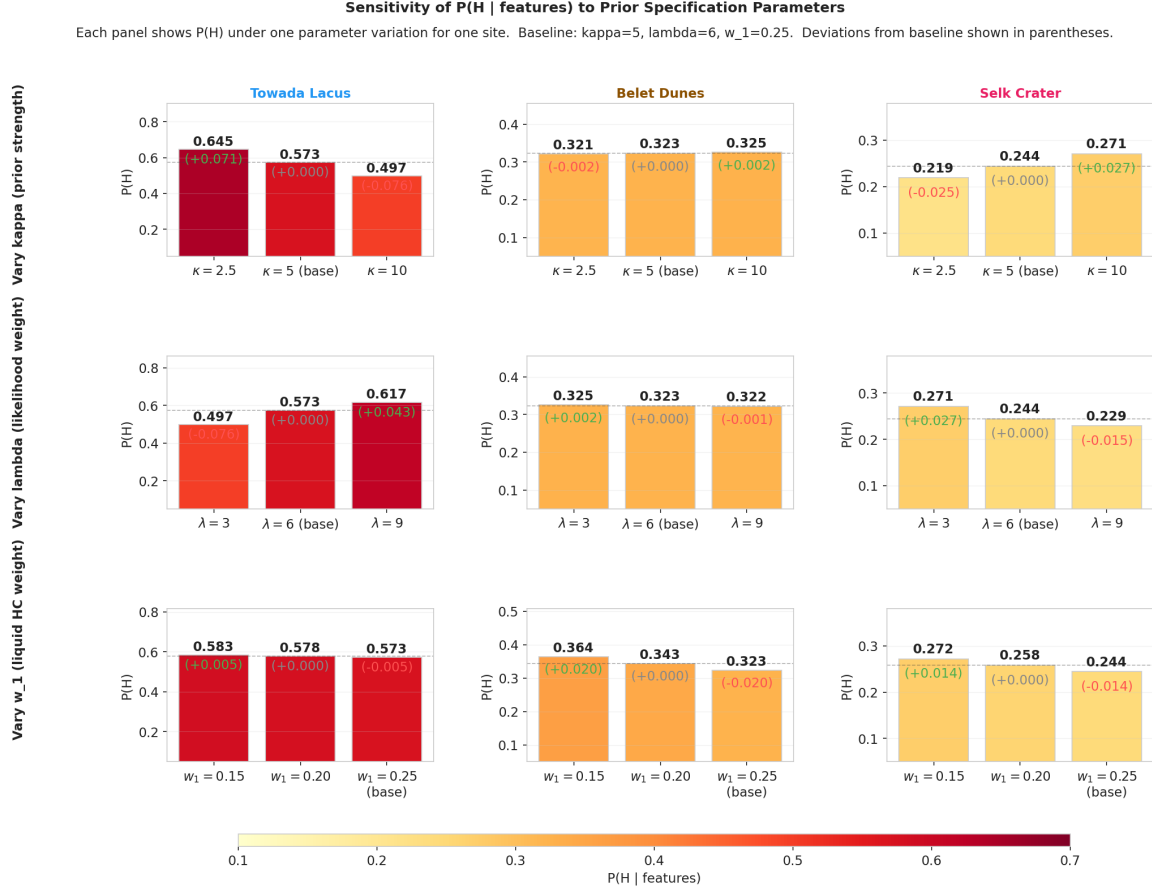
Figure 4.1: Sensitivity of P(H | \mathbf{f}) to prior specification. Each row varies one parameter; each column shows one site. Deviations \leq 0.06 for near-prior-mean sites; qualitative rankings preserved across all 27 parameter combinations.
