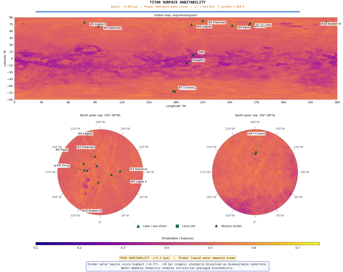
Figure 3.8: Future epoch (+5.9 Gya; red-giant ocean) posterior mean habitability. f_1 and f_8 overridden to 1.0 globally. Spatial variation reflects f_2 , f_5 , f_6 differences. Compare with Figure 3.4.
