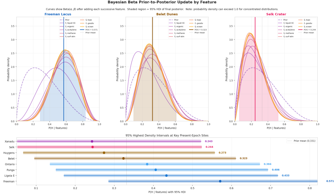
Figure 2.3: Beta prior-to-posterior update for three representative sites. Top row: each curve shows the Beta distribution after incorporating successive features, from the prior (dashed) through to the 8-feature posterior (solid). Shaded region = 95% HDI of the final posterior. Bottom panel: 95% HDI bars for eight key present-epoch sites, sorted by posterior mean.
