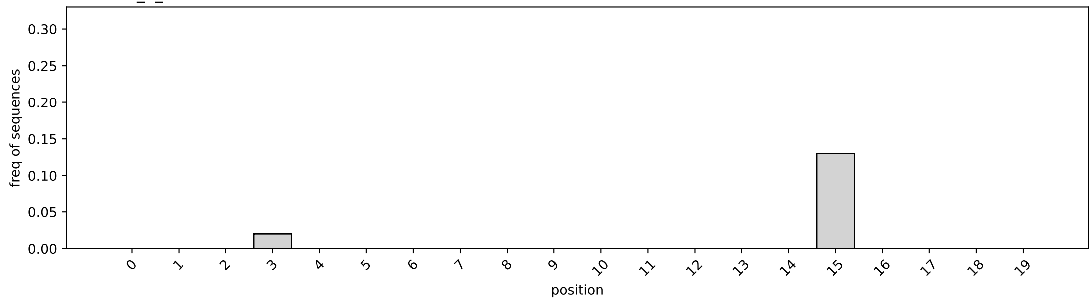
varVAMP_0_LEFT
