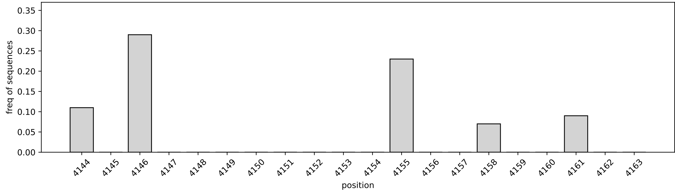
varVAMP_0_LEFT
