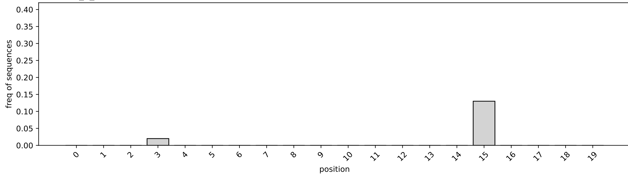
varVAMP_0_LEFT
