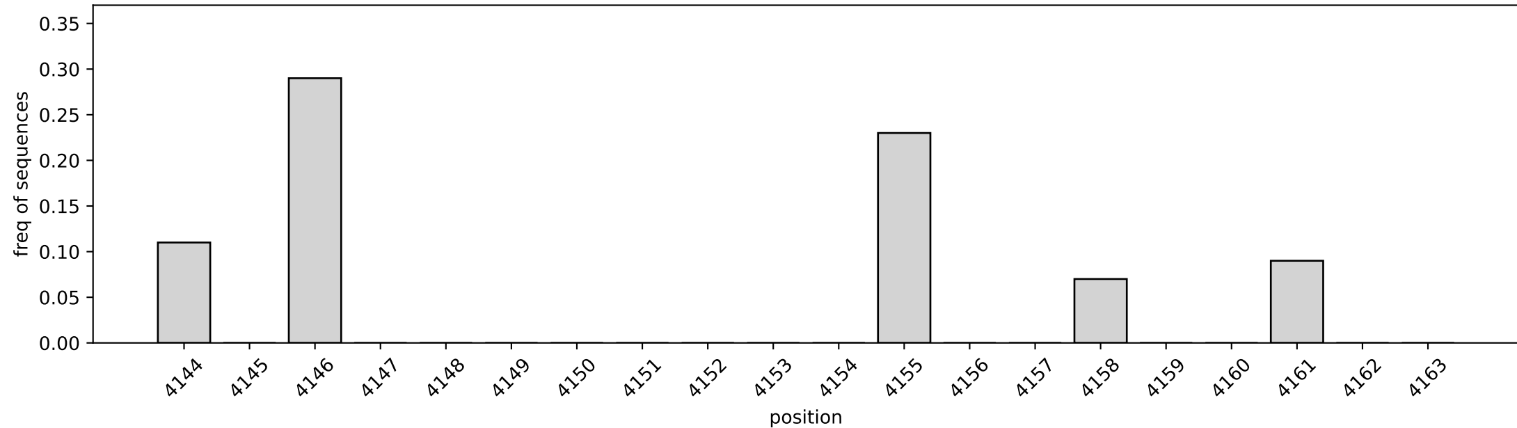
varVAMP_0_LEFT
