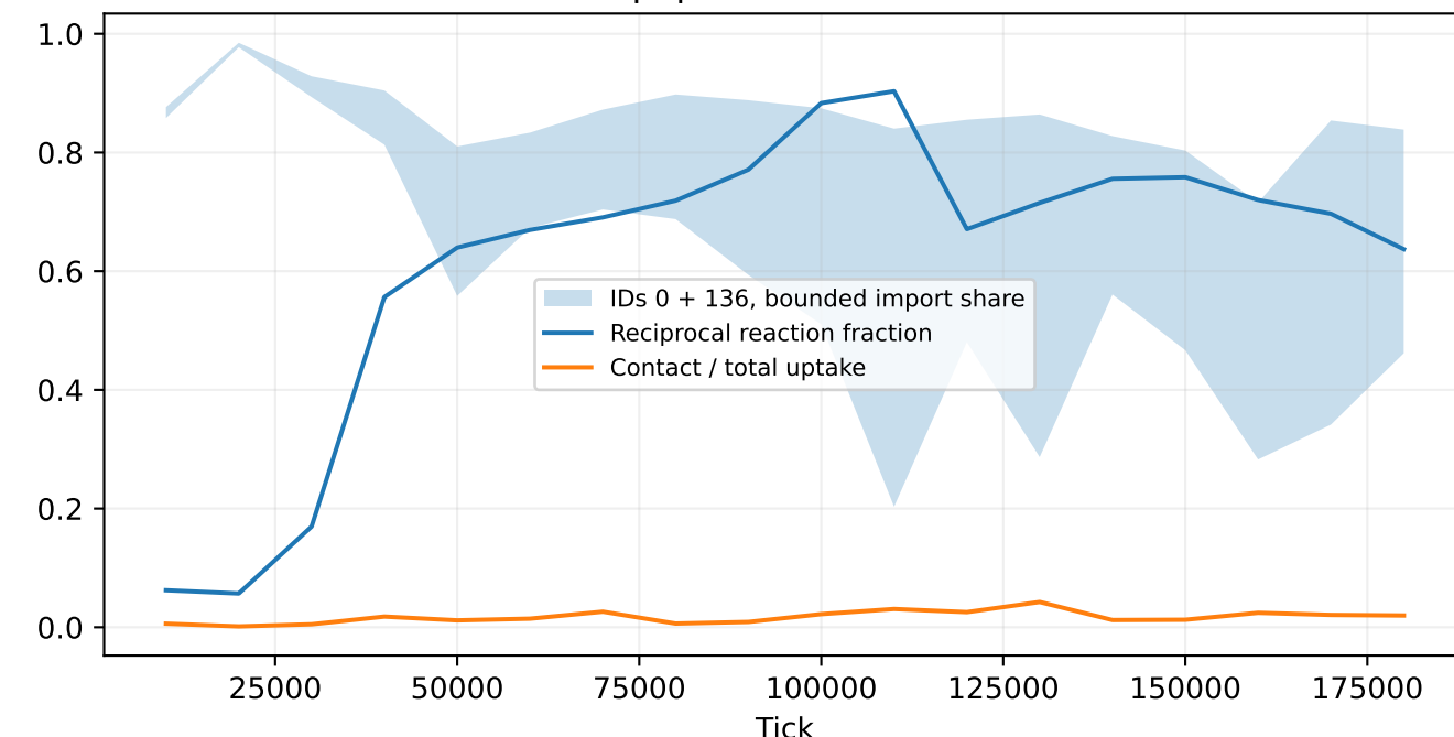
Controller responses &gt; .01 on available actions
