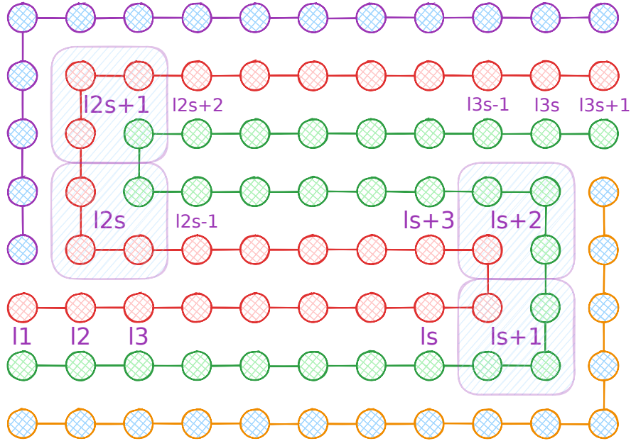
Figure 4.8: Snake Embedding technique between the folding dimension and the new dimension
