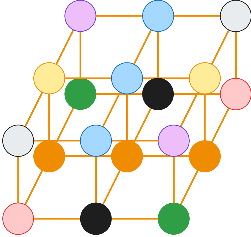
Figure 4.14: Colouring around the double sink points. The colours correspond to the colour legend of 4.12
