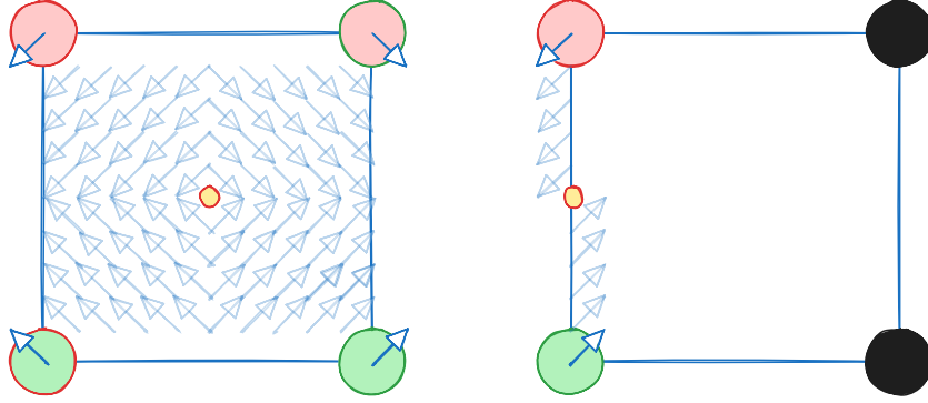
Figure 4.10: Panchromatic edge for 2 dimensions
