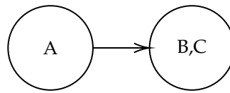
Figure 4.16: Equal solution conversion
