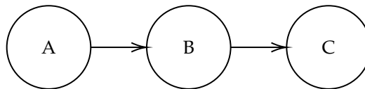
Figure 4.17: Not equal solution
