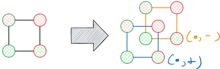
Figure 4.9: Snake Embedding technique between the folding dimension and the new dimension
