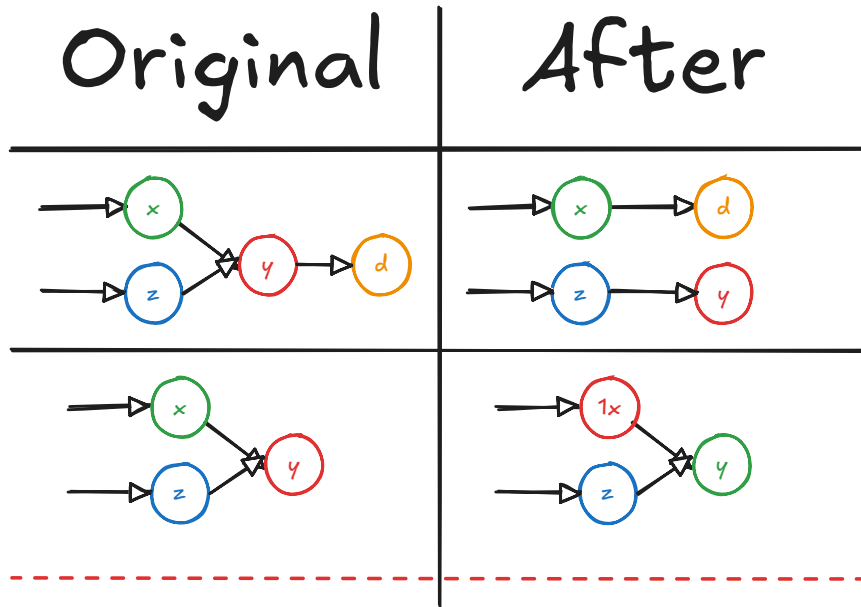
Figure 4.11: The current table shows how we deal with excess nodes. All other nodes such as sources, sinks, lines or isolated vertices stay the same.
