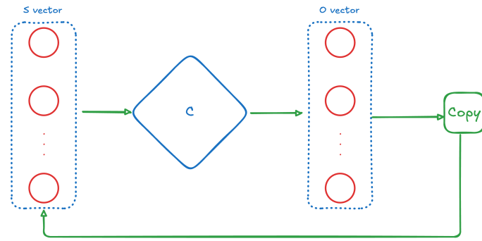
Figure 2.4.1: TARSKI construction
