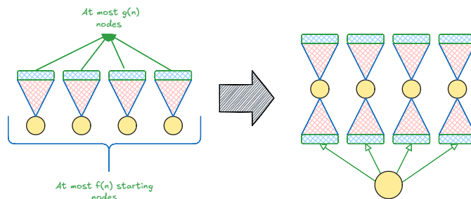
Figure 2.3.1: PolyS-Unbalanced transformation to Unbalanced
