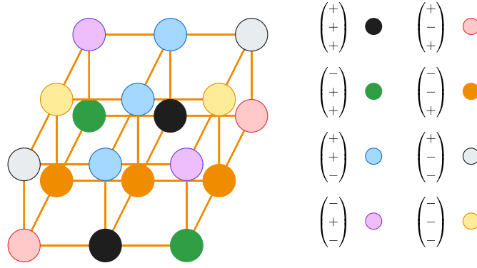
Figure 2.2.8: Colouring around the double sink points
