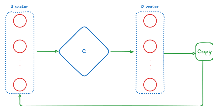
Figure 2.4.1: TARSKI construction
