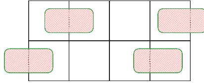
Figure 2.2.3: 1-MC with 2D\text{-SourceOrExcess}(2, 1)
