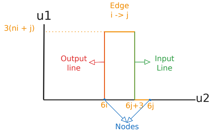
Figure 2.1.7: Edge between points i, j of the original graph, illustrates that each point comes with a pair of exponentially long lines, which we refer to as the input output lines.
