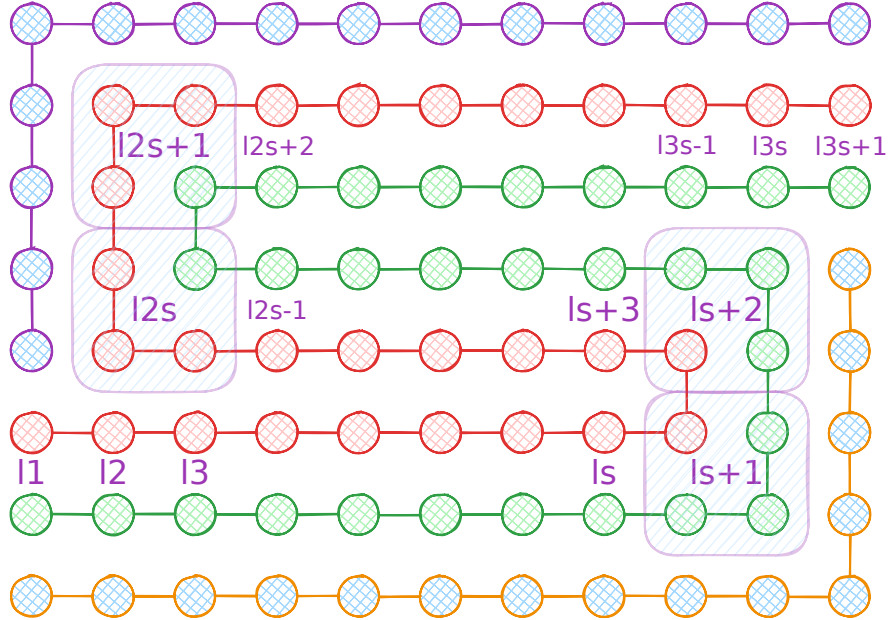
Figure 4.7: Snake Embedding technique between the folding dimension and the new dimension
