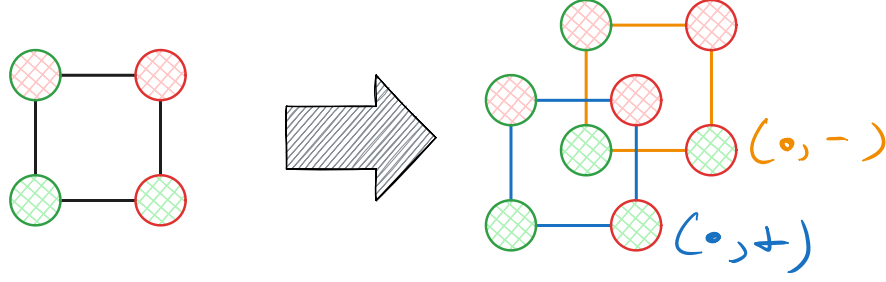
Figure 4.8: Snake Embedding technique between the folding dimension and the new dimension
