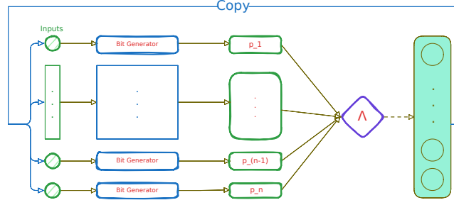
Figure 4.3: Pure Circuit construction visualisation
