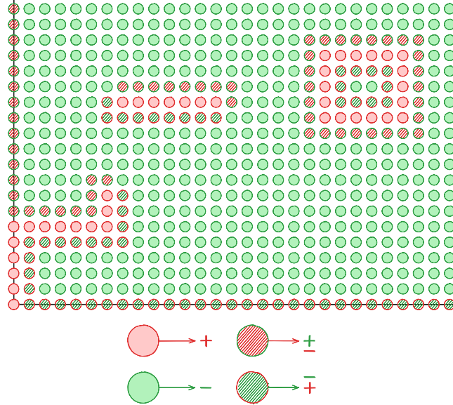
Figure 4.6: 2D EndOfLine Bipolar Colouring
