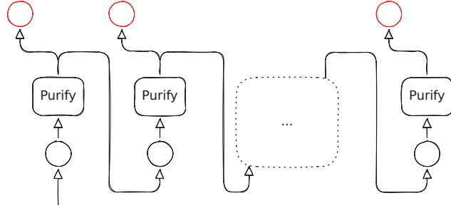
Figure 4.4: Purification gadget. The red nodes denote the outputs of the purification gadget.
