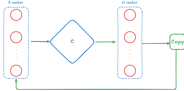
Figure 4.9: TARSKI construction
