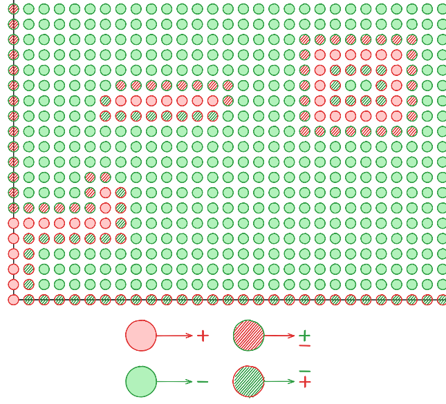
Figure 4.7: 2D EndOfLine Bipolar Colouring
