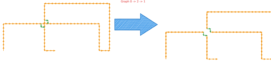
Figure 2.5: Depiction of the edge removal. Main idea is that this we keep the number of sources or sinks as well as invertible (we can trace the source or sink from the original instance), despite losing a lot of graph information.
