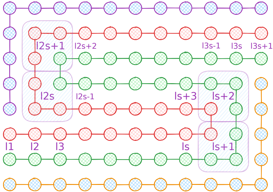
Figure 4.9: Snake Embedding technique between the folding dimension and the new dimension
