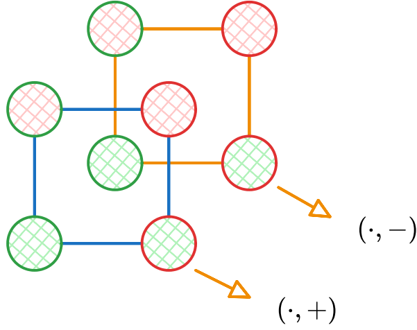
Figure 4.10: Snake Embedding technique between the folding dimension and the new dimension
