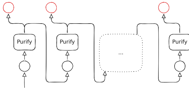
Figure 4.5: Purification gadget. The red nodes denote the outputs of the purification gadget.
