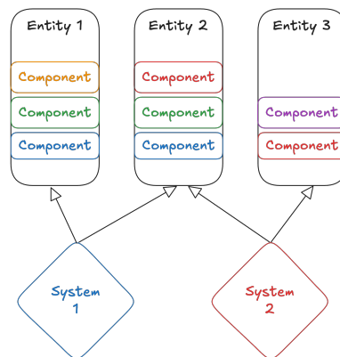
Figure 5.1: ECS visualisation implementation
