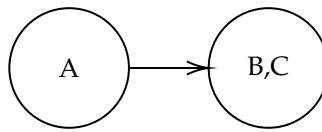
Figure 4.17: Equal solution conversion
