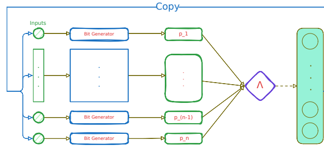
Figure 4.4: Pure Circuit construction visualisation
