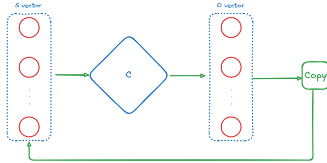
Figure 4.16: TARSKI construction
