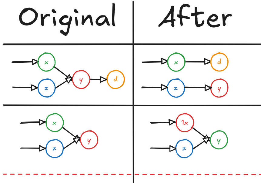
Figure 4.12: The current table shows how we deal with excess nodes. All other nodes such as sources, sinks, lines or isolated vertices stay the same.
