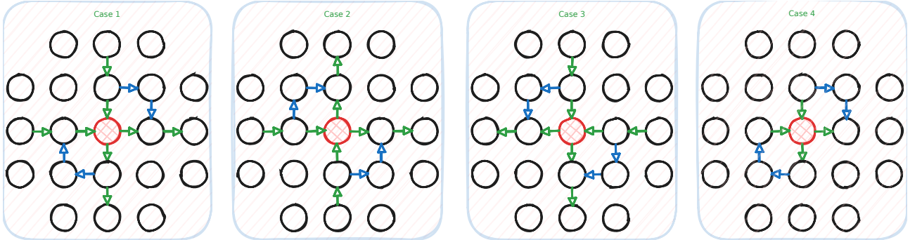
Figure 2.2: Figure redrawn from [7]
