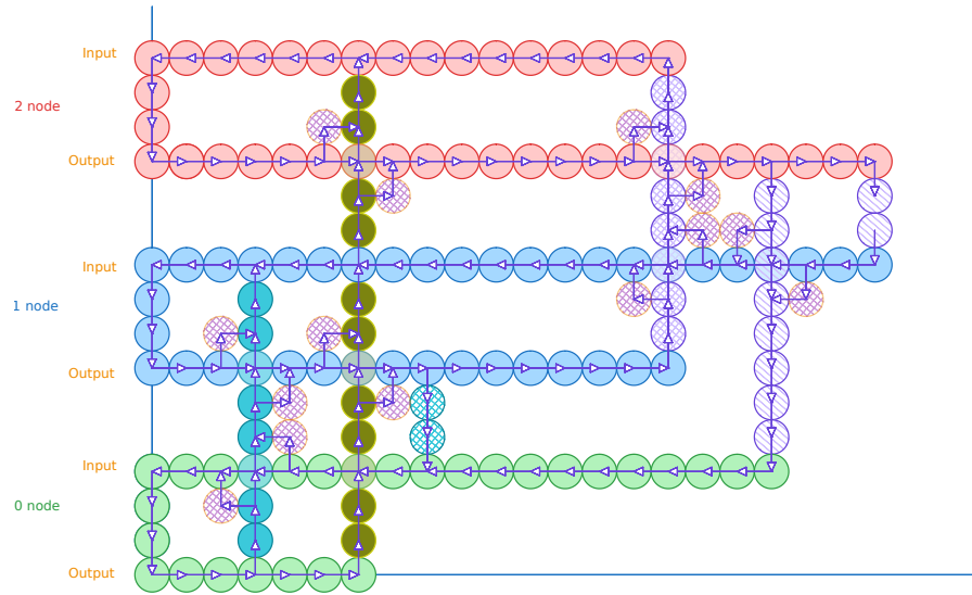
Figure 2.4: K_3 graph construction. Combinations of colours indicate an edge between the two nodes. Solid dots indicate edges from 0, crossed lines indicate edges from 1 and striped lines indicate edges from 2. We Add two coloured striped circles on the 4 degree nodes to indicate the E_n^2 edges.
