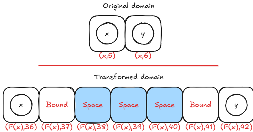
Figure 4.8: Transformed domain mapping example.
