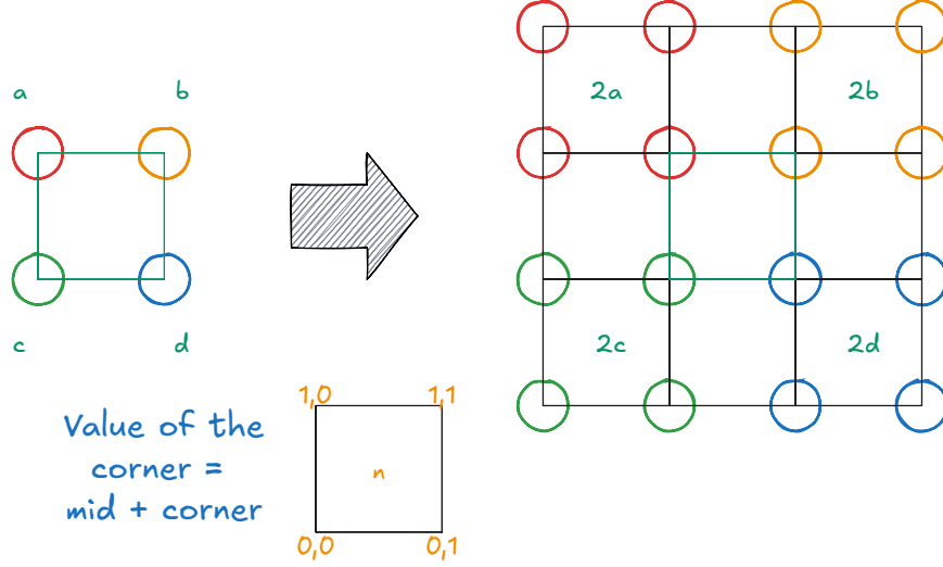
Figure 4.2: Dimension doubling. We demonstrate the example in two dimensions.
