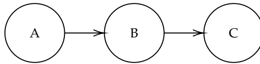
Figure 2.1.25: Not equal solution
