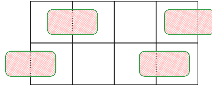
Figure 2.1.17: 1-MC with RLeafDExcess(2,1)
