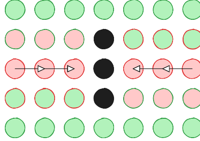
Figure 2.1.16: 2D-StrongSperner with RLeafDExcess(2,1)
