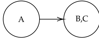
Figure 2.1.24: Equal solution conversion
