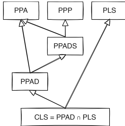
Figure 1.2.1: TFNP hierarchy. Figure re-created by [34].
