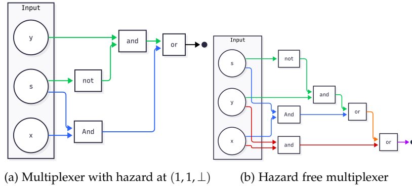
Figure 1.2.9: Hazard circuit and hazard-free circuit. Main idea is for MUX(s, x, y) , MUX(\perp, 1, 1) should be 1 by our hazard definition. We can see that when we replace s = \perp, x = 1, y = 1 to our circuits, one of them presents a hazard. Figure by [31]
