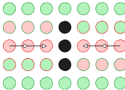
Figure 2.2.3: 2D\text{-StrongSperner} with 2D\text{-SourceOrExcess}(2,1)
