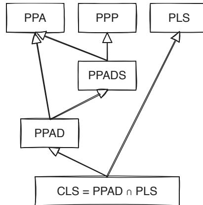
Figure 1.2.1: TFNP hierarchy. Figure re-created by [2].
