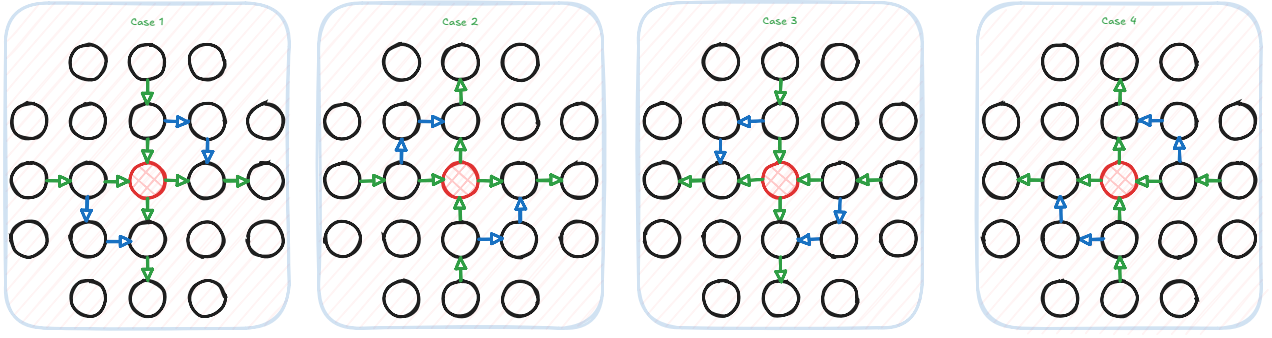
Figure 2.1.6: Edges to add for each 4 degree vertex. Figure redrawn from [16]
