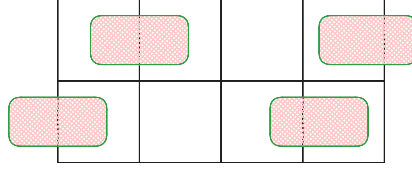
Figure 2.2.4: 1-MC with 2D\text{-SourceOrExcess}(2,1) at the double sink points
