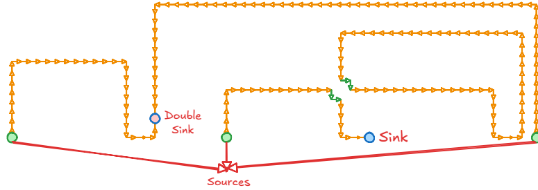
Figure 2.2.2: 2D\text{-SourceOrExcess}(2,1) example. Figure not drawn to scale
