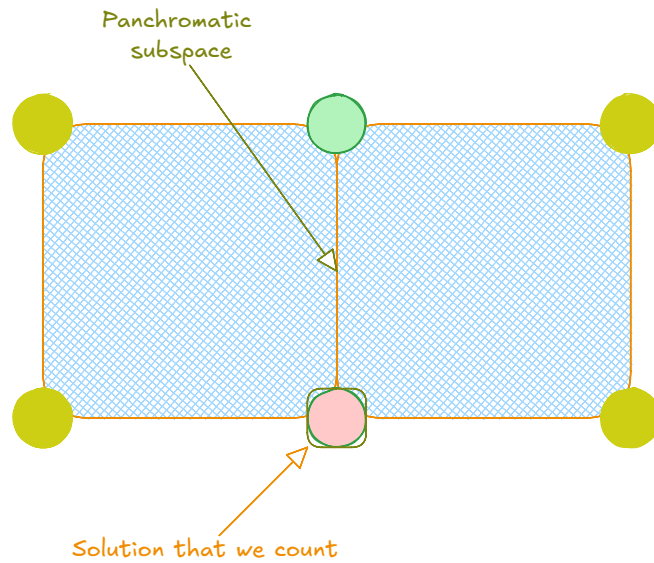
Figure 2.2.5: Panchromatic edge counting example
