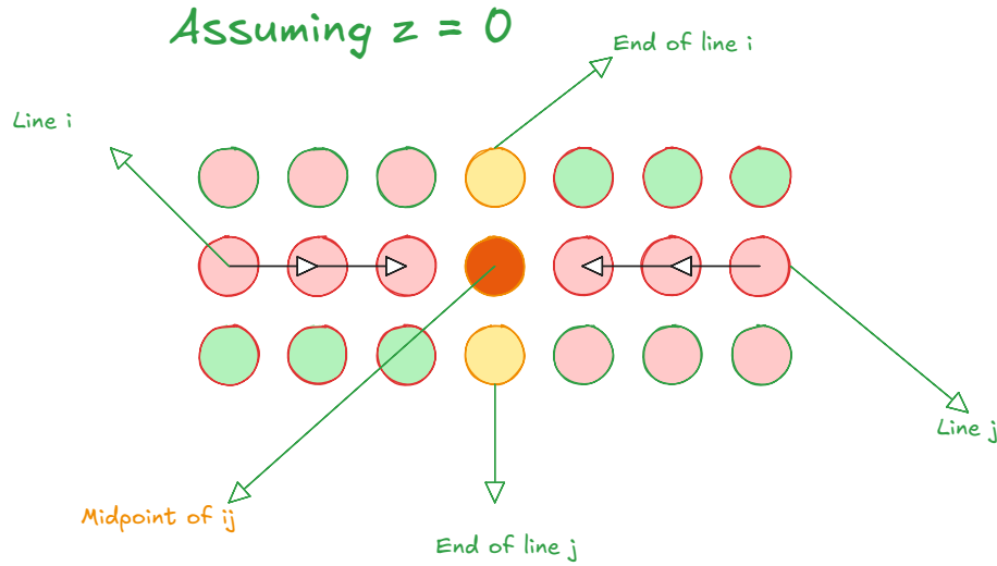
Figure 2.2.6: Double sink depiction from a 2D point of view
