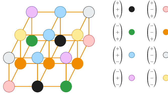
Figure 2.2.9: Colouring around the double sink points
