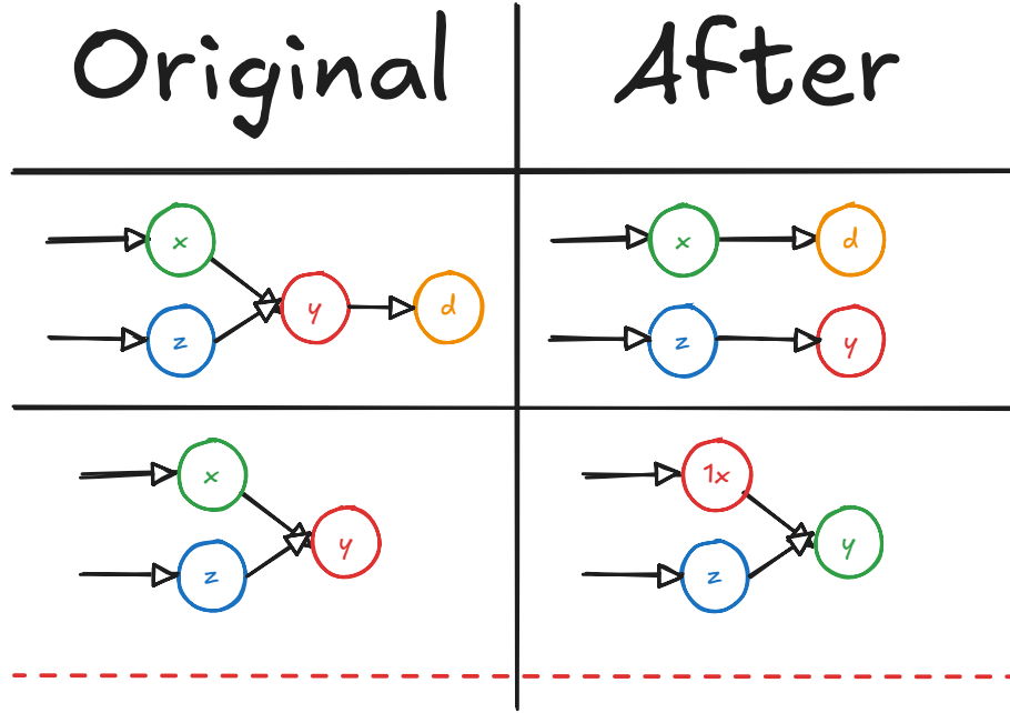
Figure 2.1.16: The current table shows how we deal with excess nodes. All other nodes such as sources, sinks, lines or isolated vertices stay the same.
