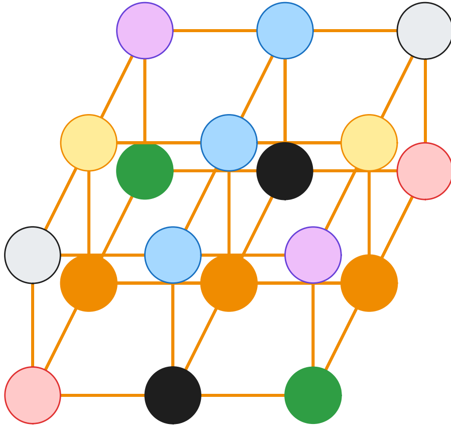
Figure 2.1.19: Colouring around the double sink points. The colours correspond to the colour legend of 2.1.17
