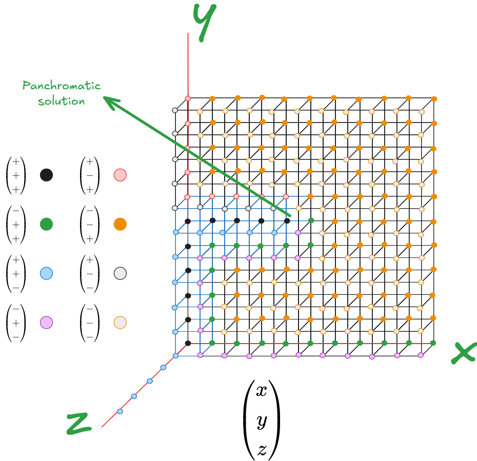
Figure 2.1.17: Colouring example based on the proposed circuit
