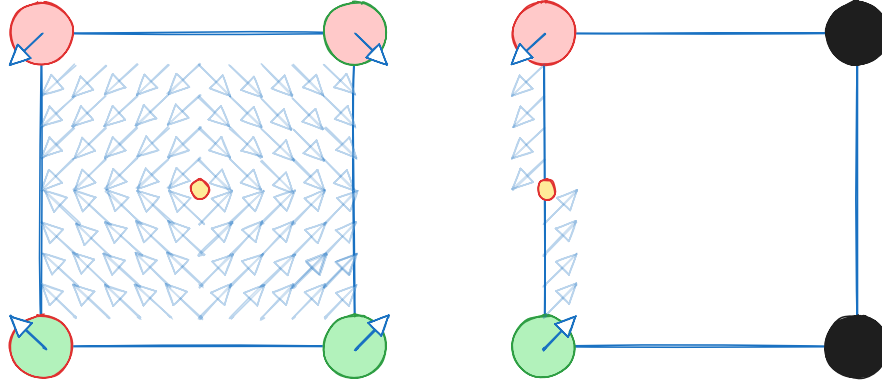
Figure 2.1.15: Panchromatic edge for 2 dimensions
