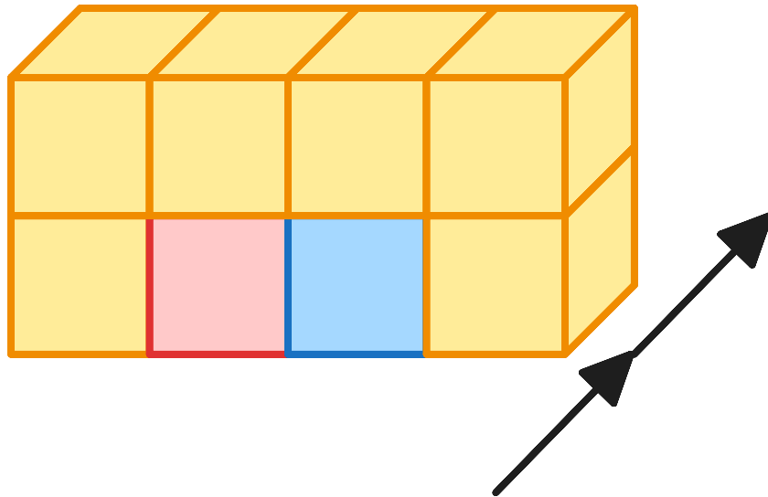
Figure 2.1.18: Example colouring where the arrow denotes the direction. In between the red and blue cubes in the bottom corners we have the positive line. The brown cubes around denote the negative labels
