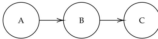
Figure 2.1.22: Not equal solution
