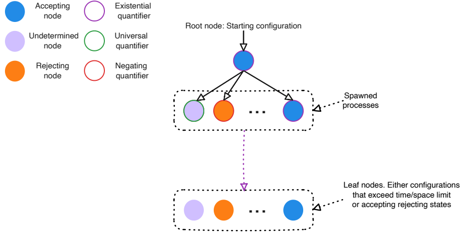
Figure 1.2.9: Computation tree of an ATM with labellings. We can observe that we start with an initial configuration and for each child, we end up in different states and configurations that have different accepting conditions. In the leafs of our tree, we may have accepting, rejecting or do not know configurations. What the \tau operator does is propagating the state from the leafs, all the way up to the root
