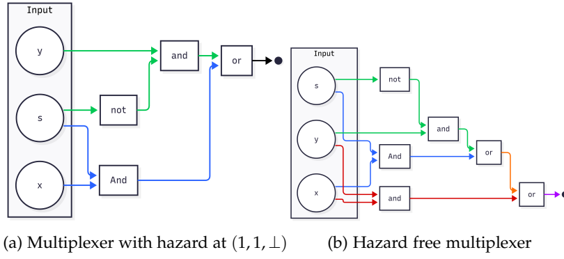
Figure 1.2.8: Hazard circuit and hazard-free circuit. Main idea is for MUX(s, x, y) , MUX(\perp, 1, 1) should be 1 by our hazard definition. We can see that when we replace s = \perp, x = 1, y = 1 to our circuits, one of them presents a hazard. Figure by [30]
