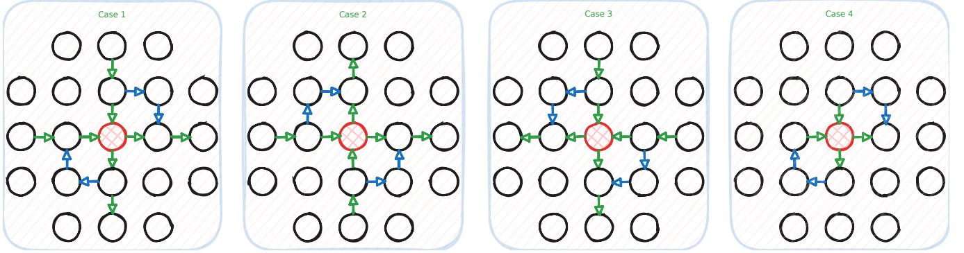
Figure 2.1.6: Edges to add for each 4 degree vertex. Figure redrawn from [12]
