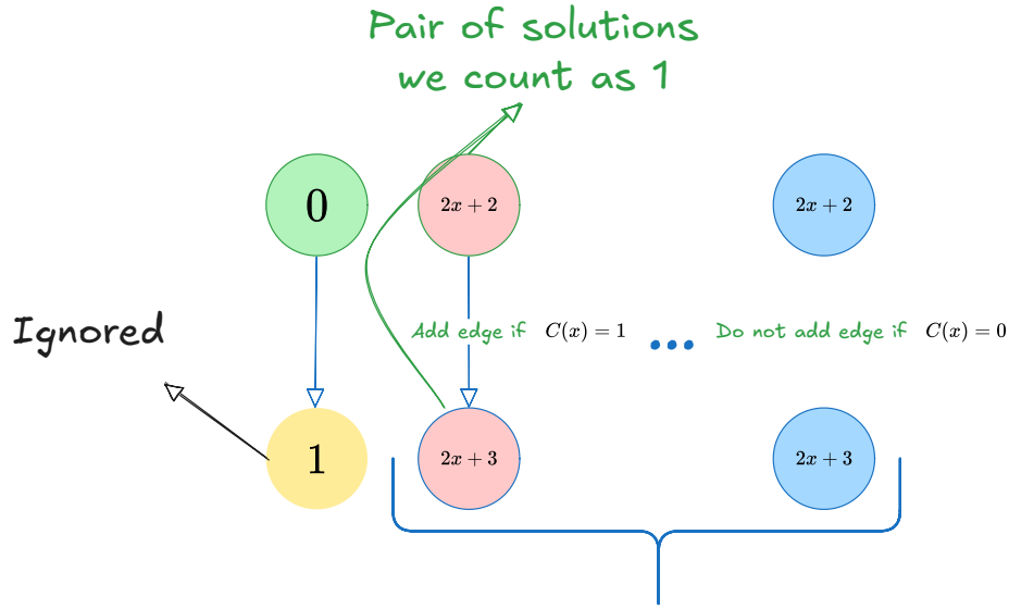
Figure 1.2.7: #CircuitSAT to ((\#EndOfLine) - 1)/2
