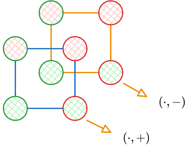
Figure 2.1.14: Panchromatic squares between the folded dimension and the new dimension
