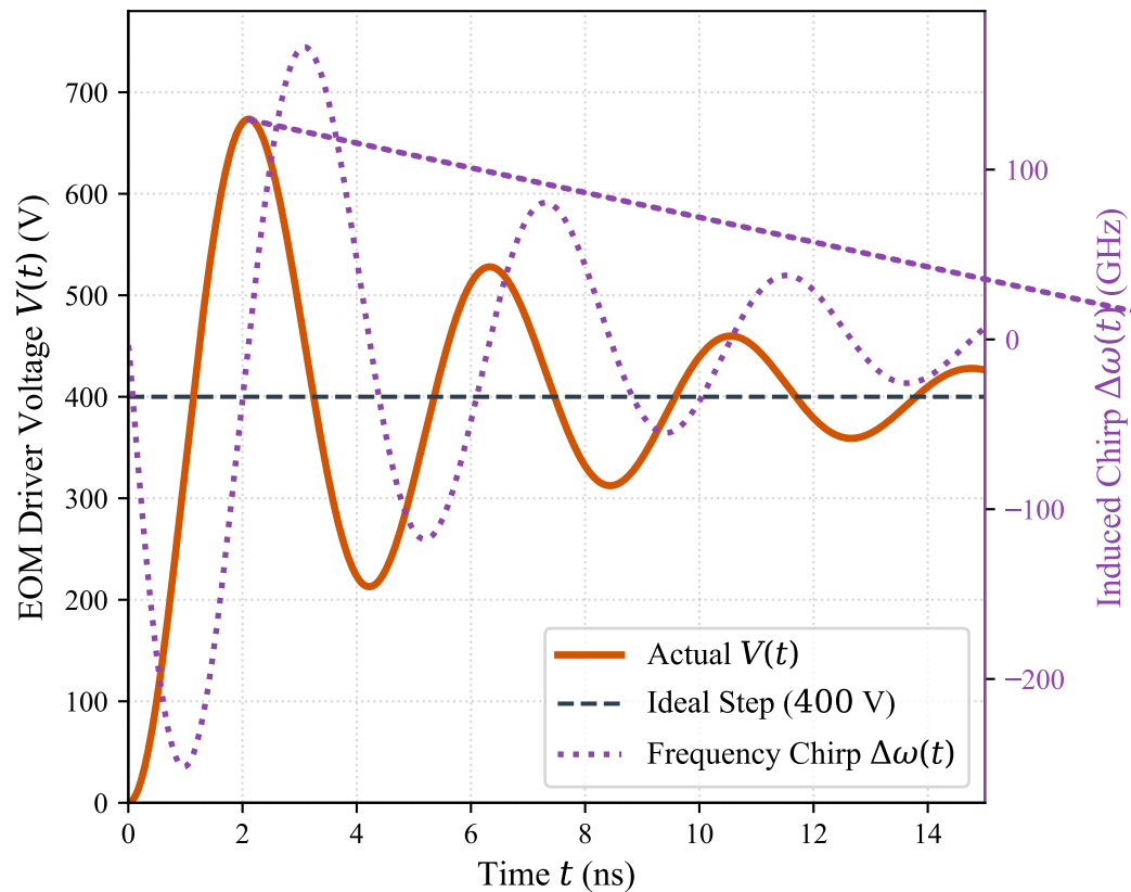
(a) EOM Ringing and Dynamic Chirp
