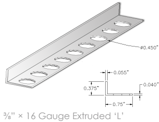
3/8" x 16 Gauge Extruded 'L'
