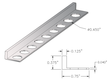
3/8" x 1/8" Extruded 'L'
