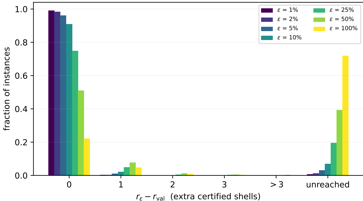
What tolerating \varepsilon bias buys over the validity radius
