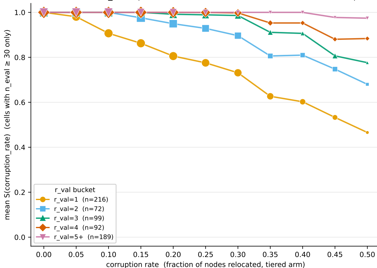
Tiered arm: r_{\text{val}} separates survival on the re-binned axis, same as flip
