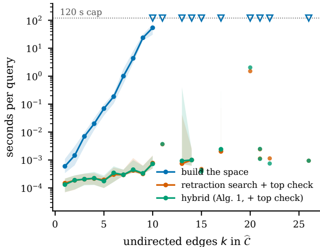
(a) Cost against k on 256 instances
