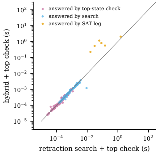
(b) Retraction search against the hybrid, per instance
