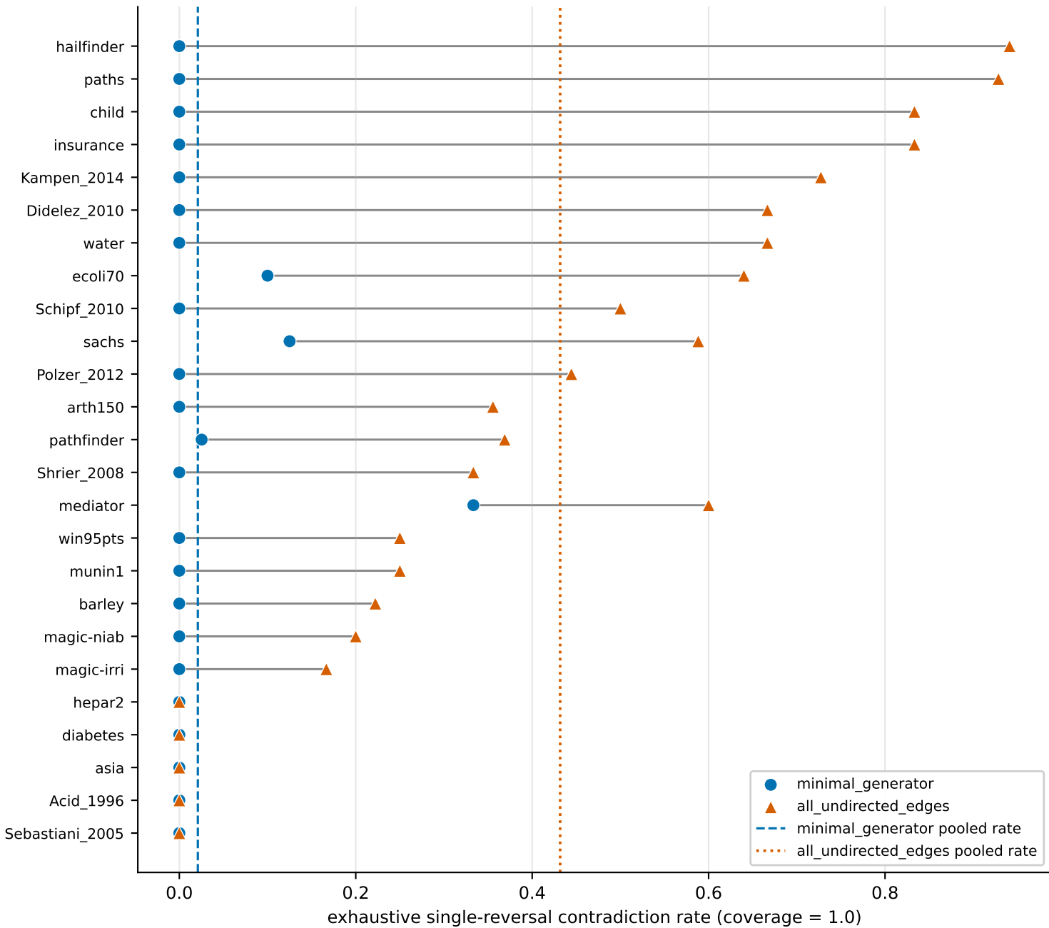
Contradiction rate under two knowledge models, paired per network
