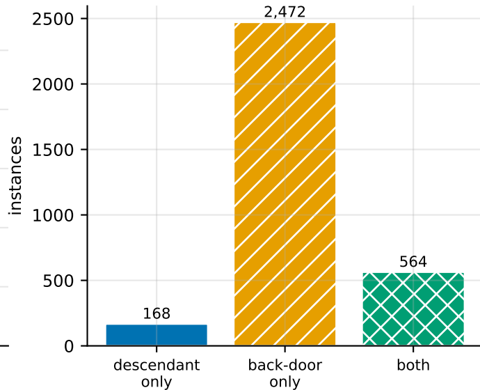
Bounds: the back-door mode carries most of the coverage coverage of the lower bound which mode supplies the bound
